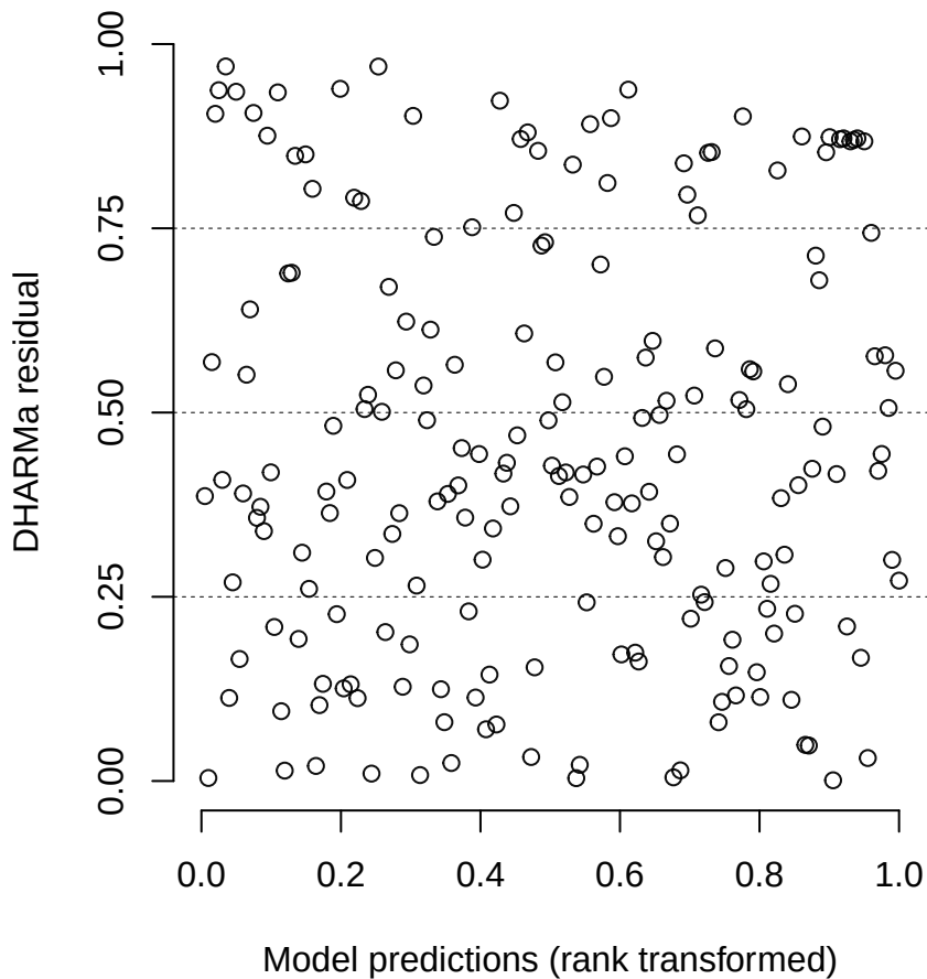
DHARMA residual vs. predicted Some quantile regressions failed
