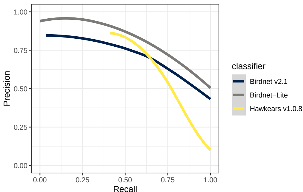
Figure 4: Performance of each acoustic classifier on the Jasper dataset.
