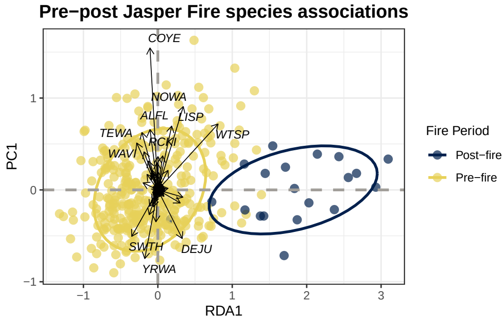
Figure 11: Community matrix of species associations before and after the Jasper 2024 fire on the VALLEY5 and TEKARRA transects. Movement along RDA1 reflects the direction and magnitude of fire-related change in species composition. PC1 captures residual variation in species composition that is not explained by fire period reflecting the background ecological variability among sites.
