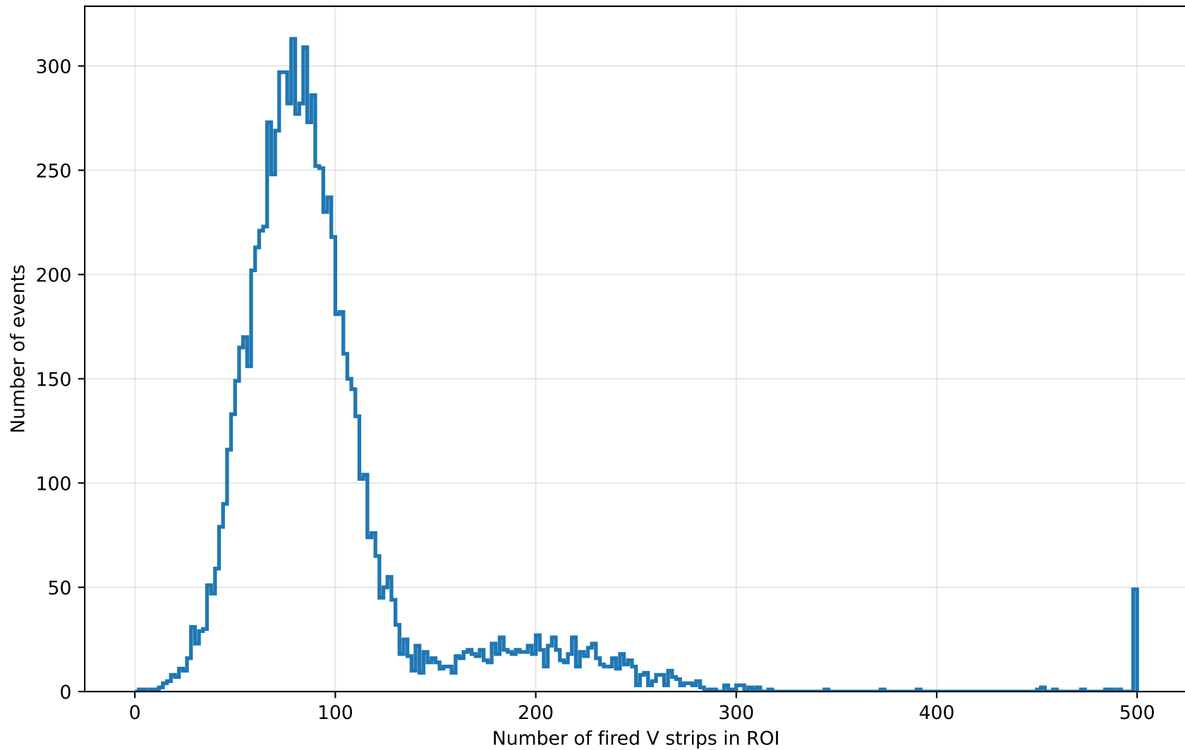
Distribution of fired V strips in ROI
