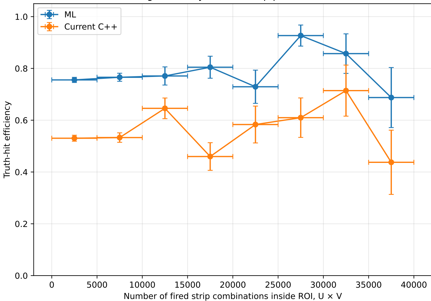
Hit-finding efficiency vs fired strip product inside ROI
