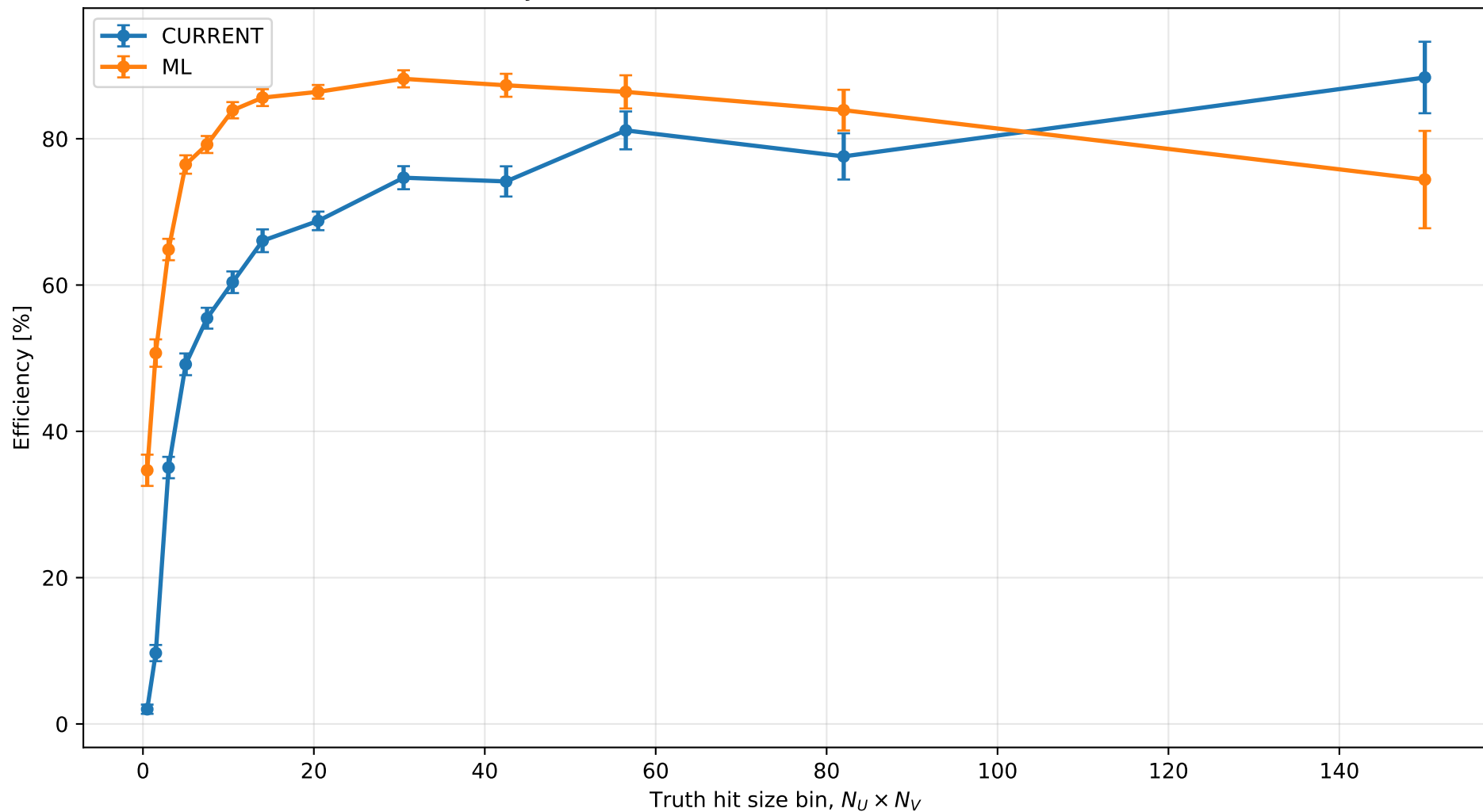
Efficiency vs binned truth-hit size Only bins with at least 1 truth events are shown
