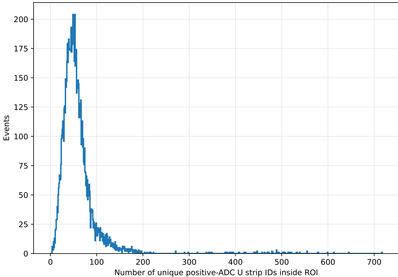
Unique positive-ADC U strip count per event inside ROI
