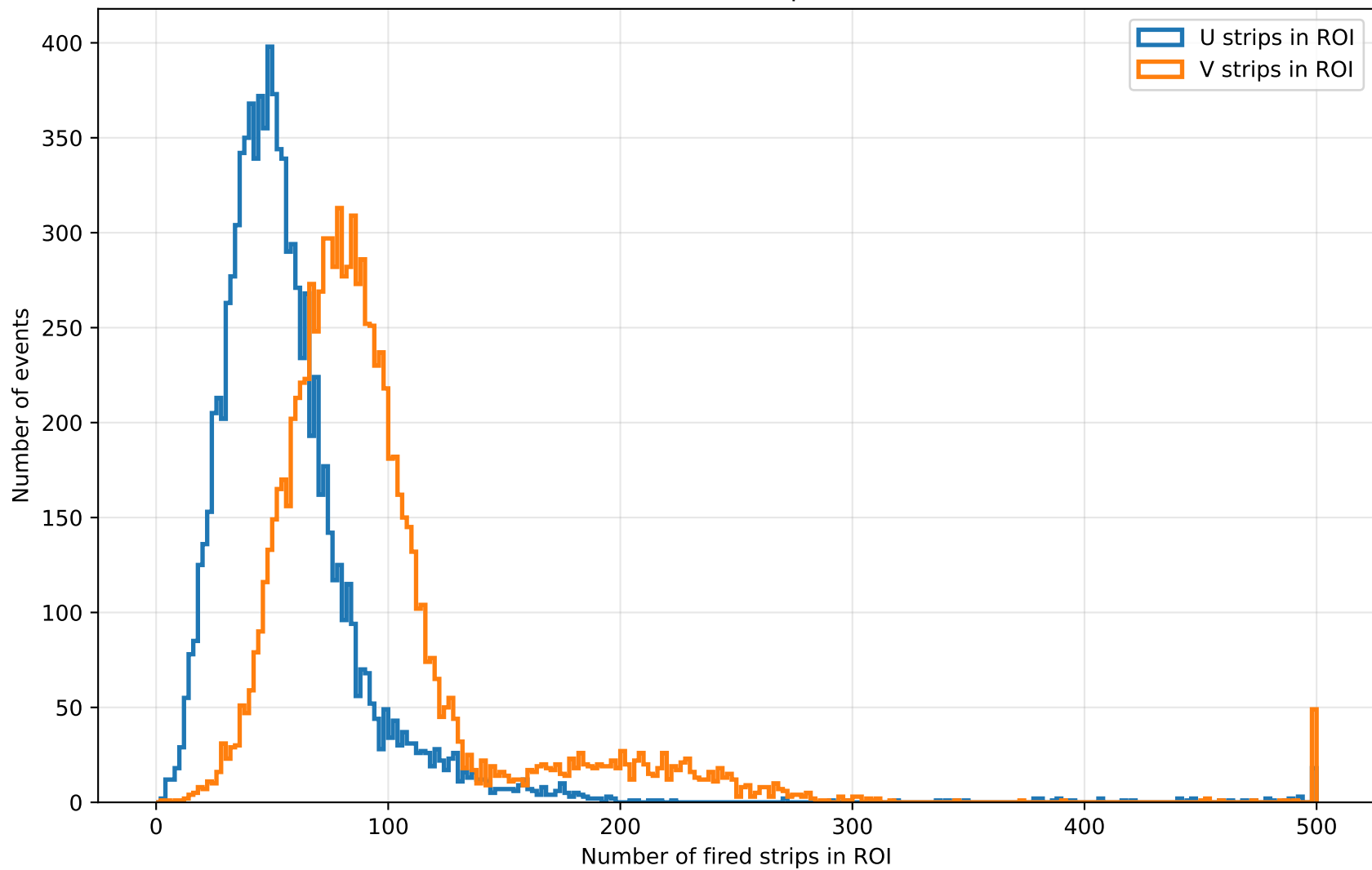
Fired U and V strips in ROI
