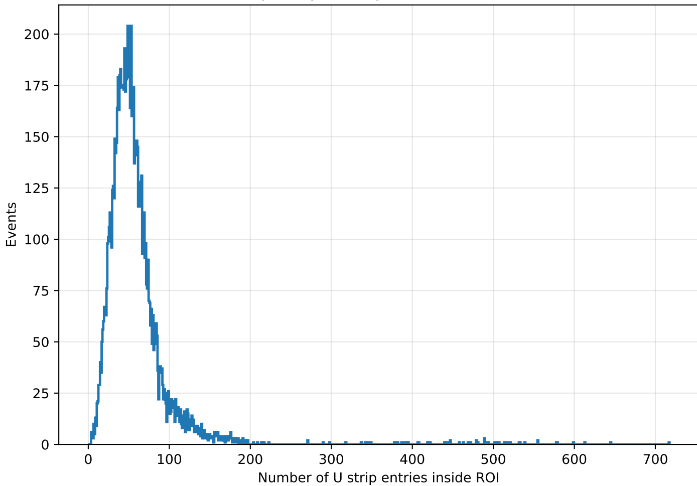
U strip-entry count per event inside ROI
