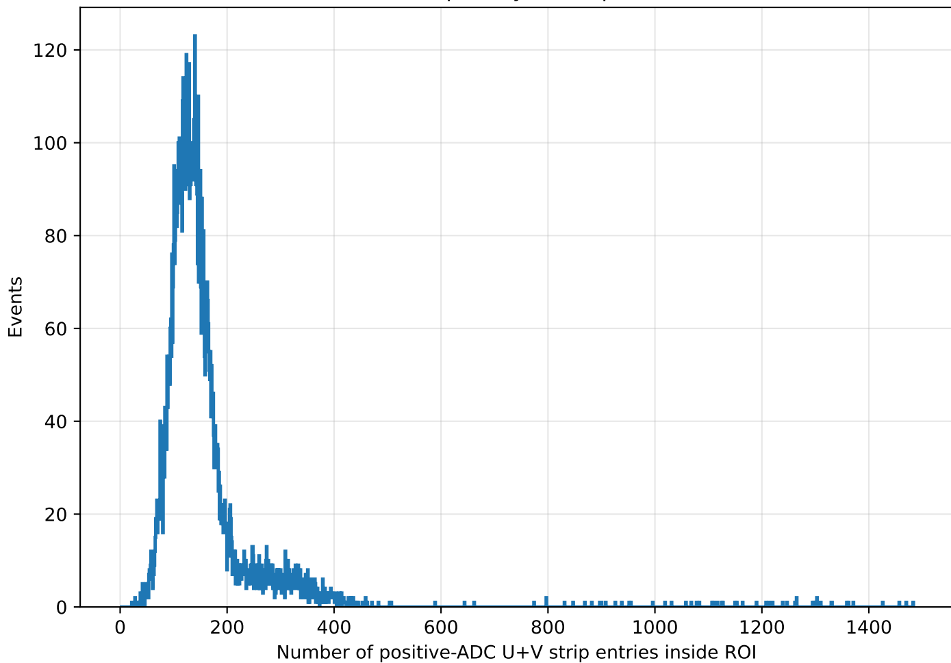
Positive-ADC U+V strip-entry count per event inside ROI
