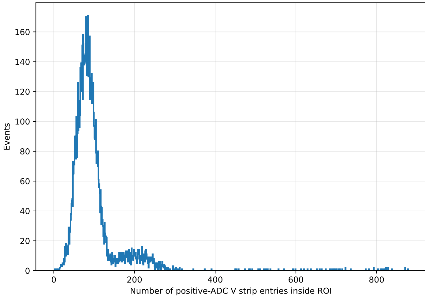
Positive-ADC V strip-entry count per event inside ROI
