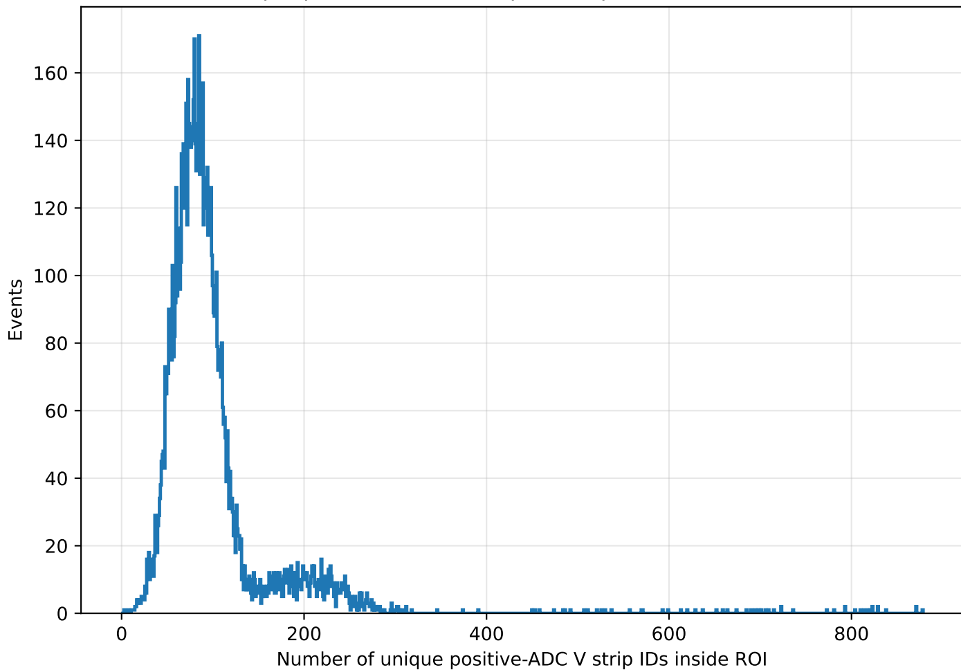
Unique positive-ADC V strip count per event inside ROI
