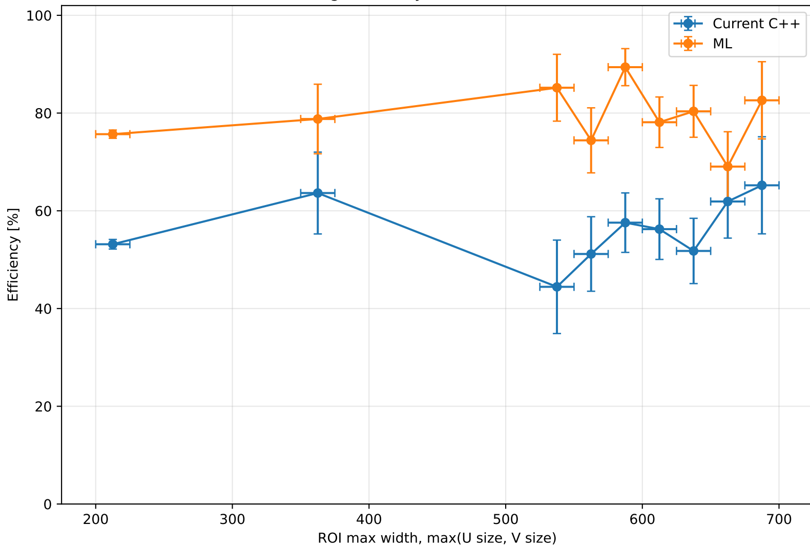
Hit-finding efficiency vs ROI maximum width
