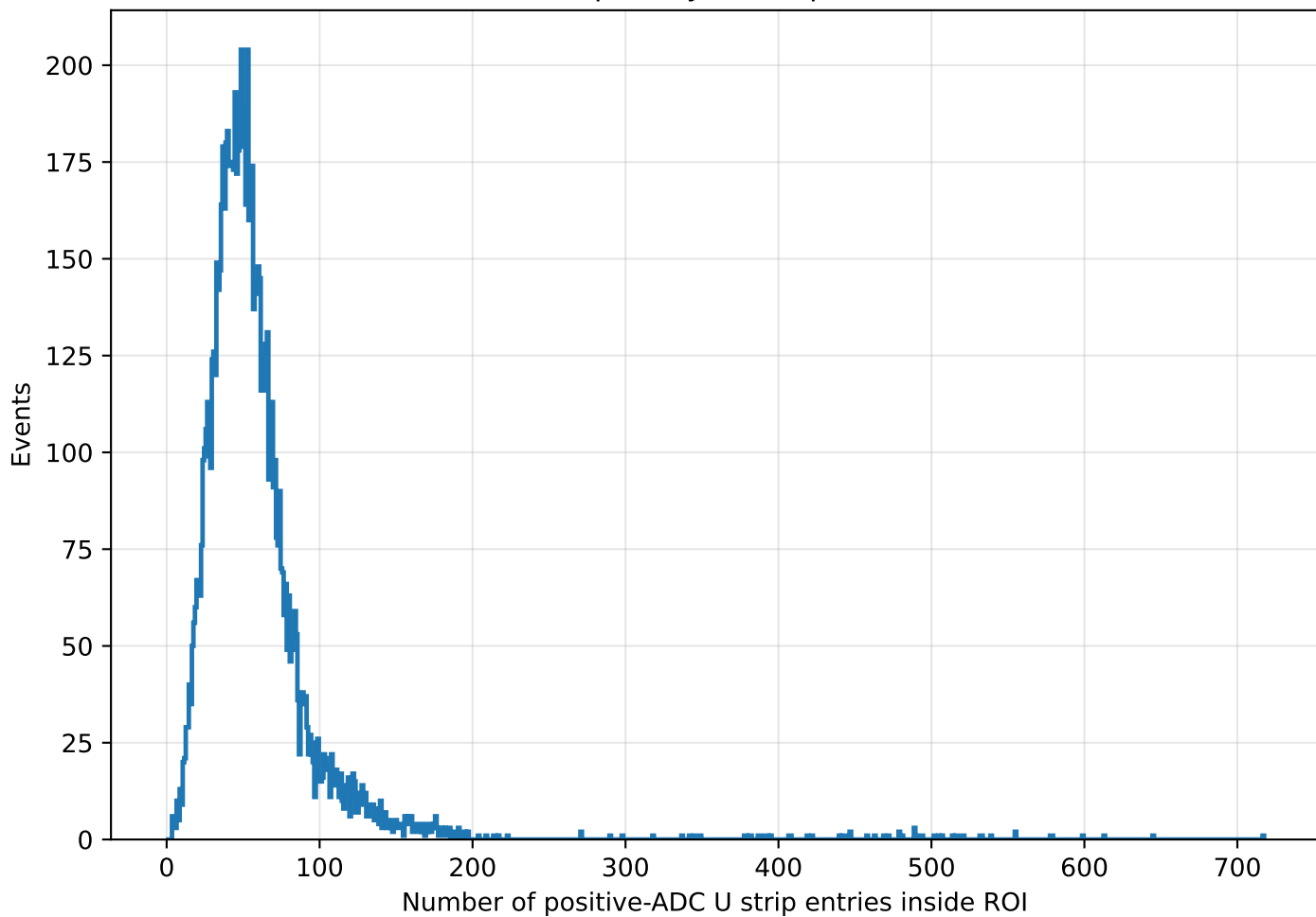
Positive-ADC U strip-entry count per event inside ROI
