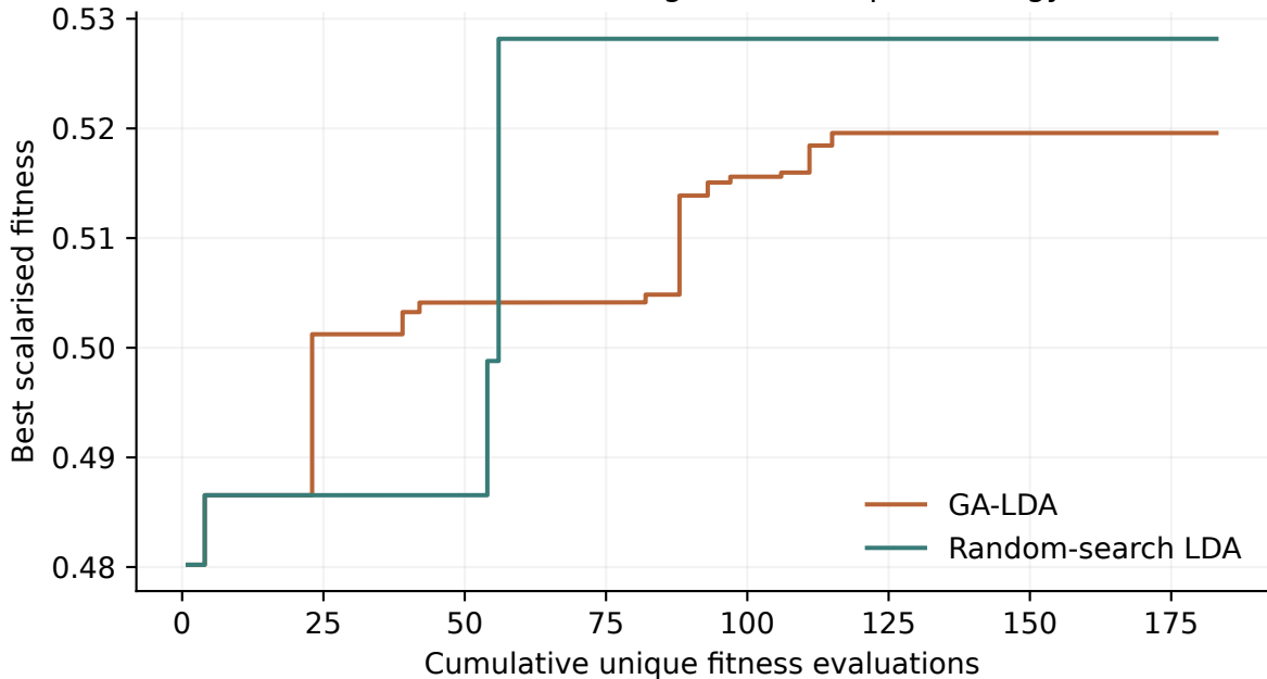
Matched search budget: one run per strategy
