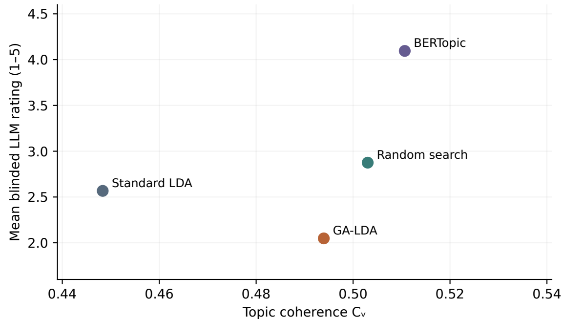
Coherence and automated interpretability
