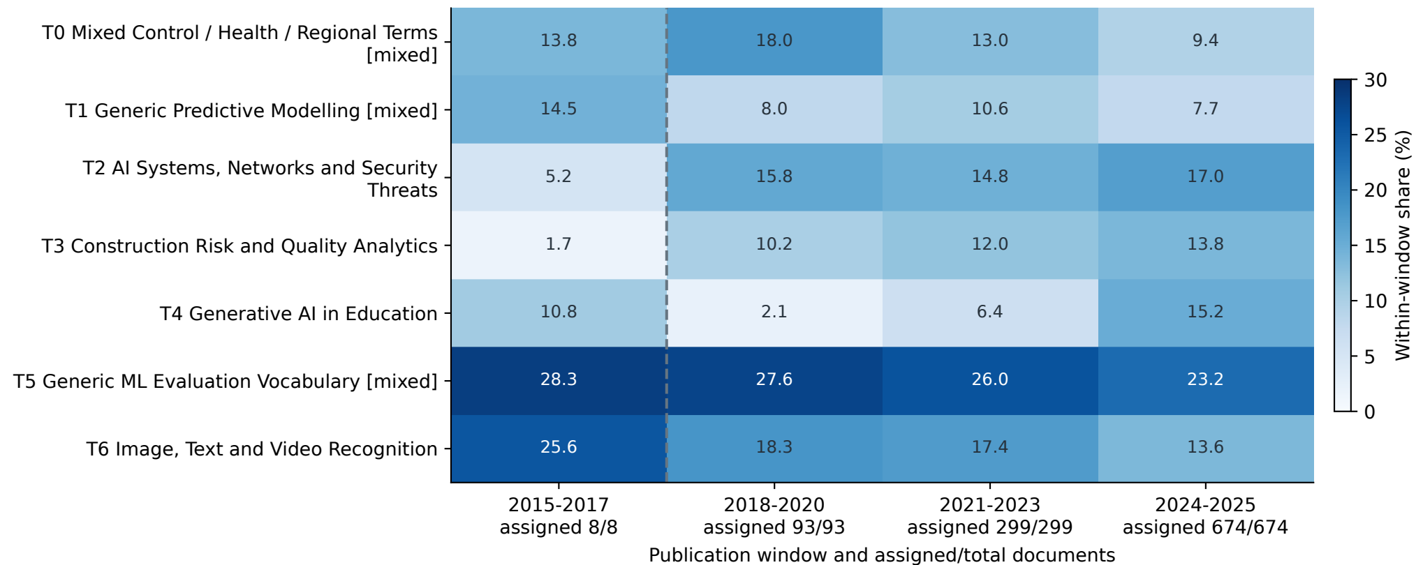
GA-LDA: mean topic mass, all documents 2015-2017 is descriptive only (n=8)
