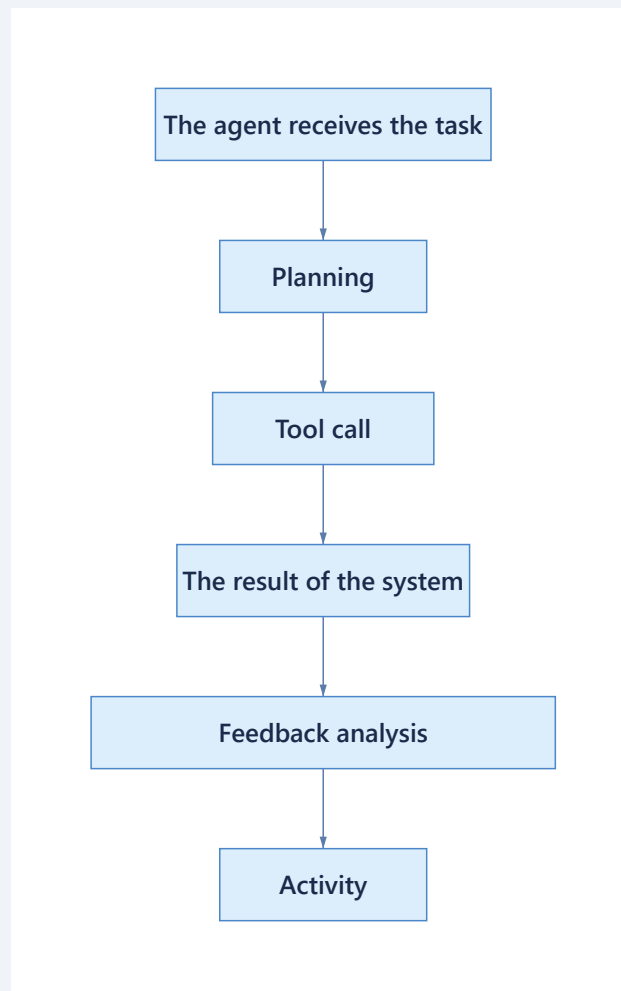
Figure 6.7: Feedback from the external system in the agent cycle (Tool Use - observe).
