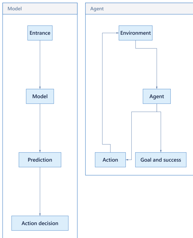
Figure 6.1: Contrast of the model as a passive predictor and the agent as an active participant in the feedback loop with the environment. In the modern age, we are witnessing how this evolution is taking place at an accelerated rate. Large language models (LLM), which in their beginning were primarily complex statistical models of language, today are increasingly incorporated into architectures that enable them to act as agents. By connecting to external tools, data sources and action capabilities, they cease to be purely text generators and become the core of reasoning within more complex agents capable of planning and executing tasks. This confirms that the development path of artificial intelligence is directed from the creation of sophisticated analytical tools towards the formation of autonomous, rational and purposeful stakeholders in the digital and physical world. ## 6.2 Programmable language: the role of the application programming interface (API) as a bridge Application
