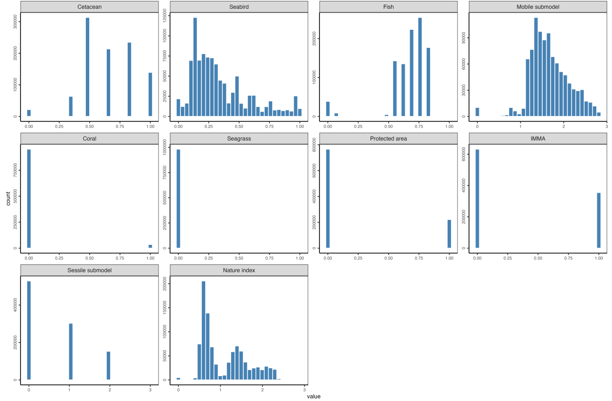
Figure 4: Data score histograms comprising nature index in Greater North Sea
