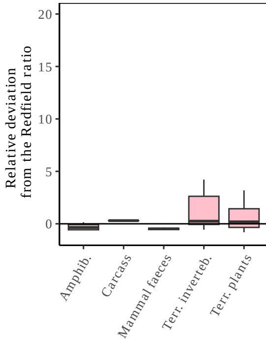
N:P of exported subsidies
