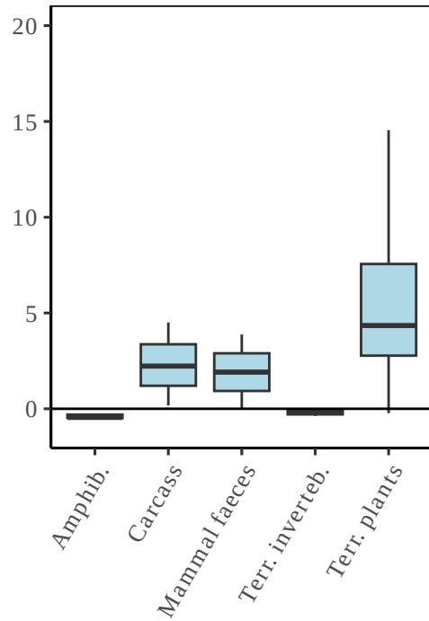
C:N of exported subsidies
