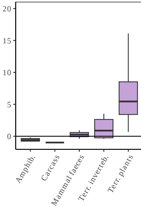
C:P of exported subsidies
