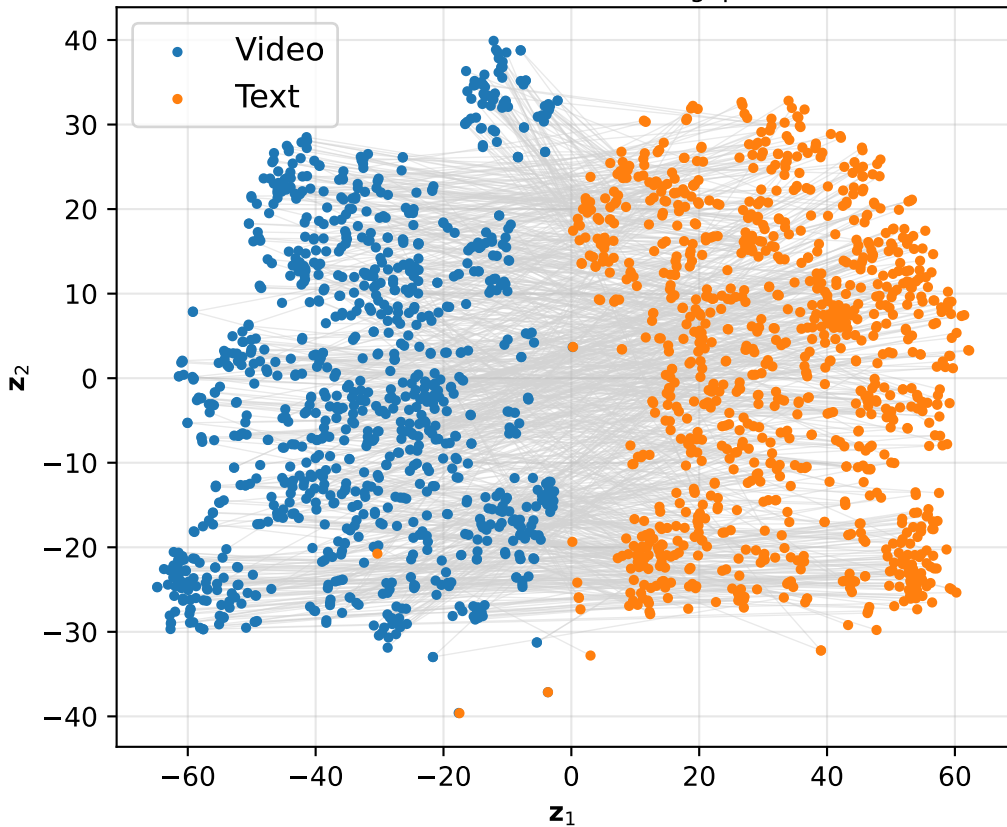
Qwen3VL-Instruct-8B ( ||\vec{\Delta}_{\text{gap}}|| = 0.41 )
