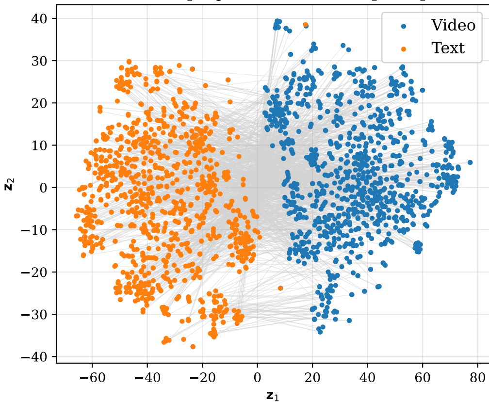
2D tSNE projection (No EOL prompt)
