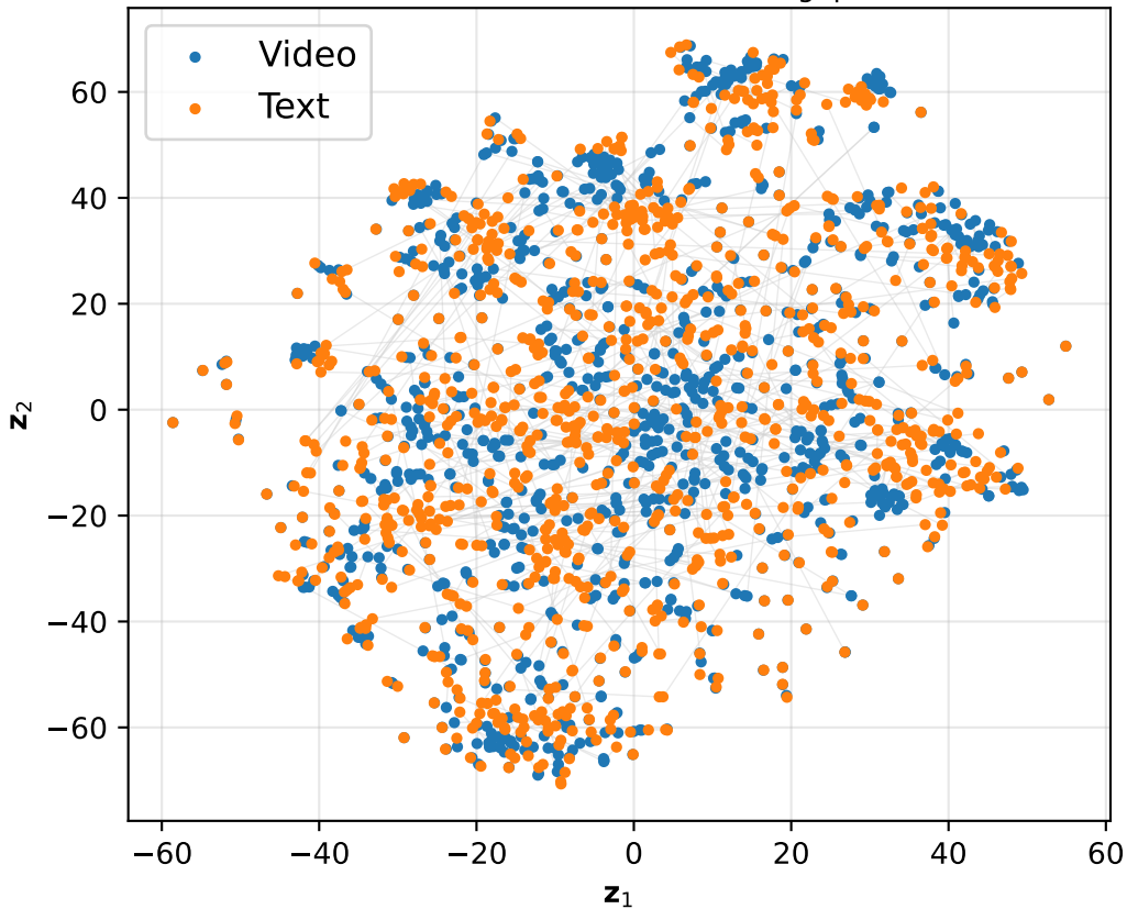
Qwen3VL-Embedding-8B ( ||\vec{\Delta}_{\text{gap}}|| = 0.23 )
