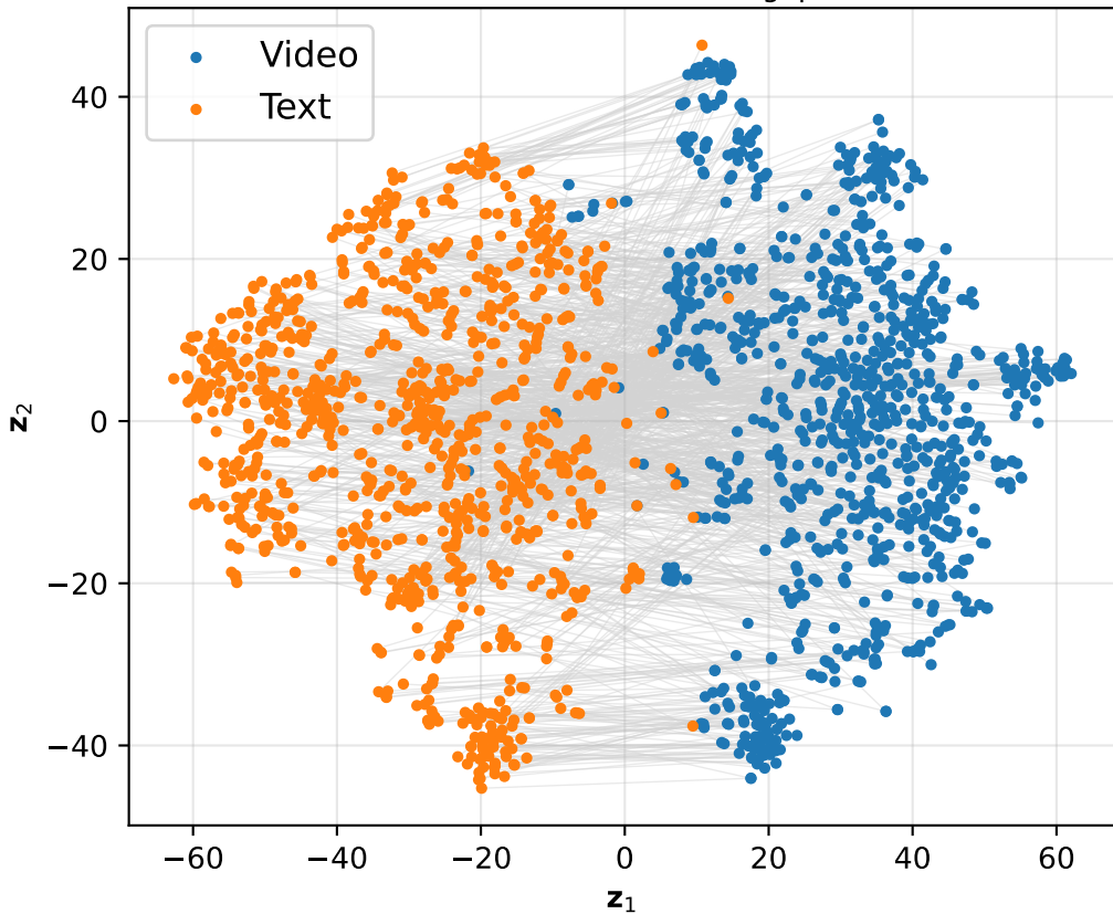
Qwen3VL-Instruct-8B ( ||\vec{\Delta}_{\text{gap}}|| = 0.61 )
