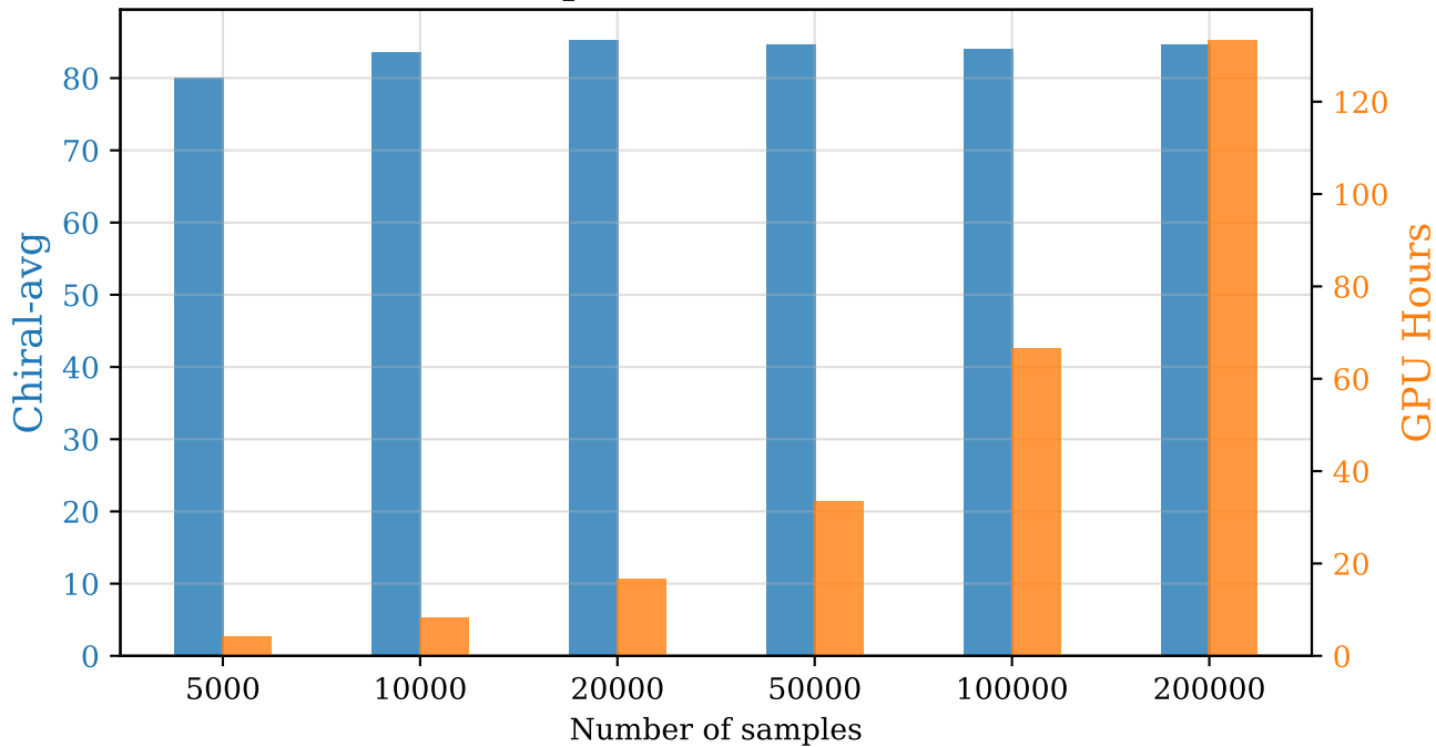
Impact of data size
