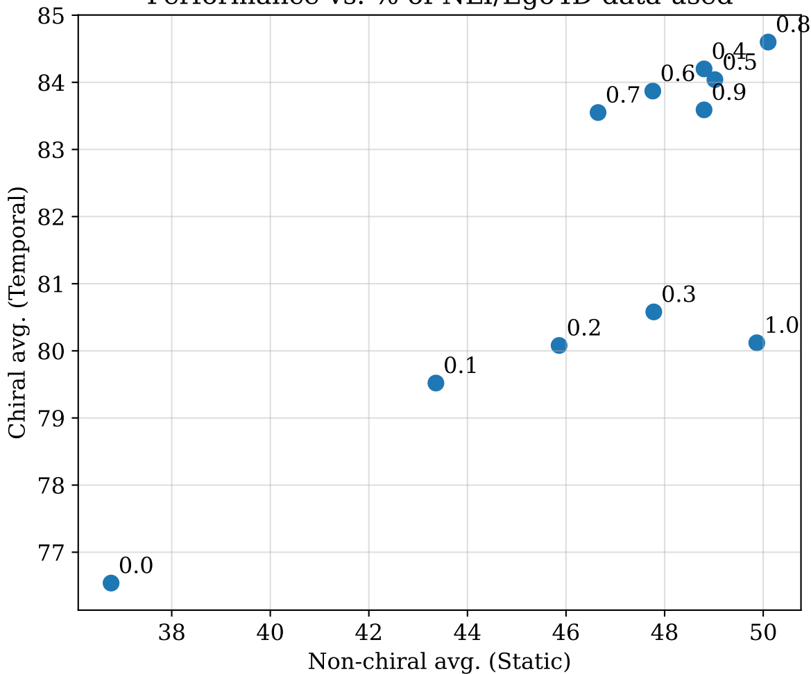
Performance vs. % of NLI/Ego4D data used
