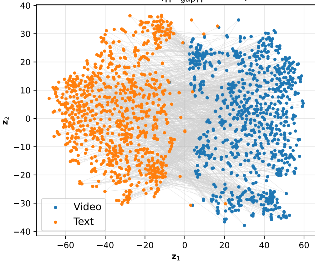
tarsier7b ( ||\vec{\Delta}_{\text{gap}}|| = 0.44 )
