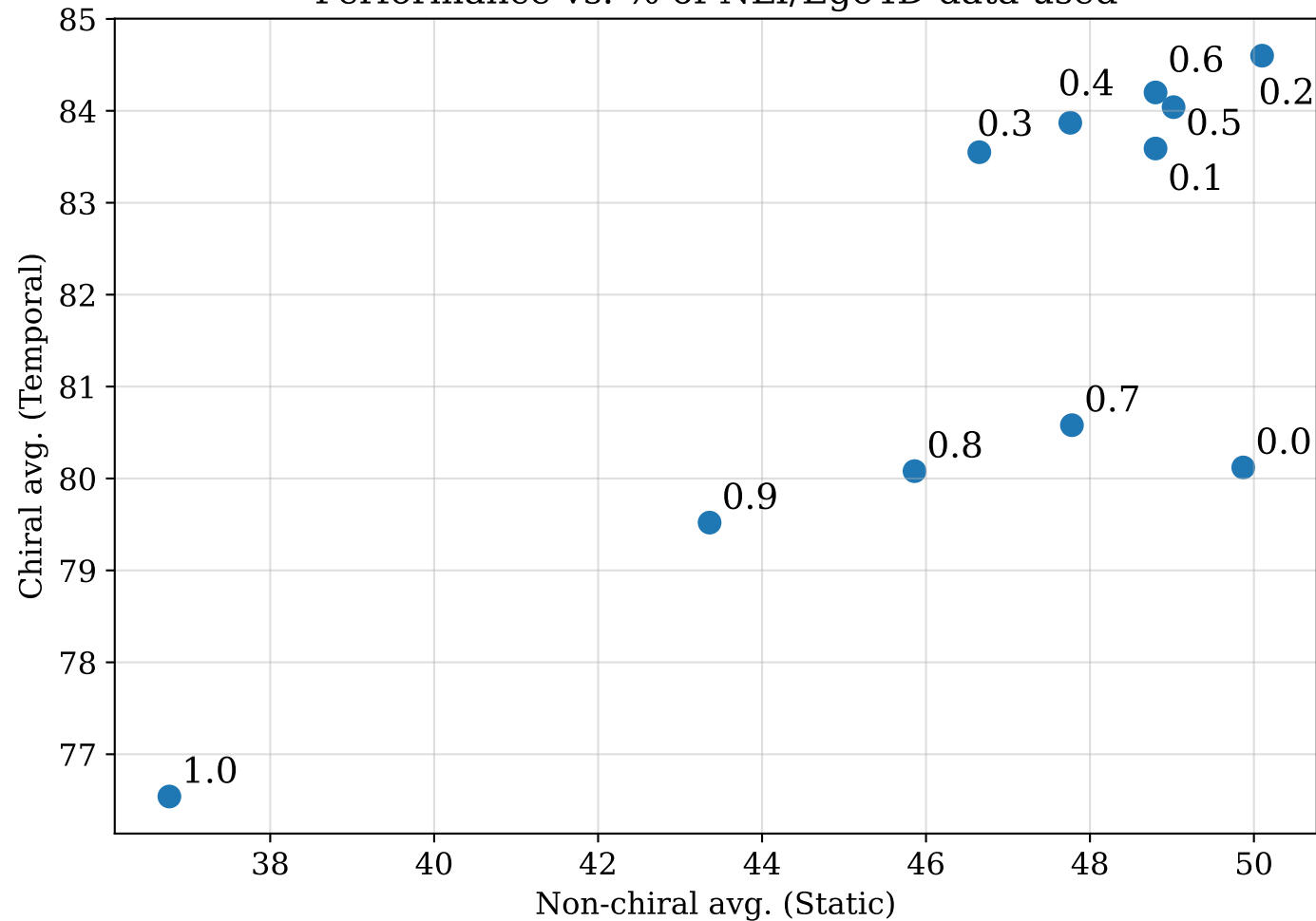
Performance vs. % of NLI/Ego4D data used
