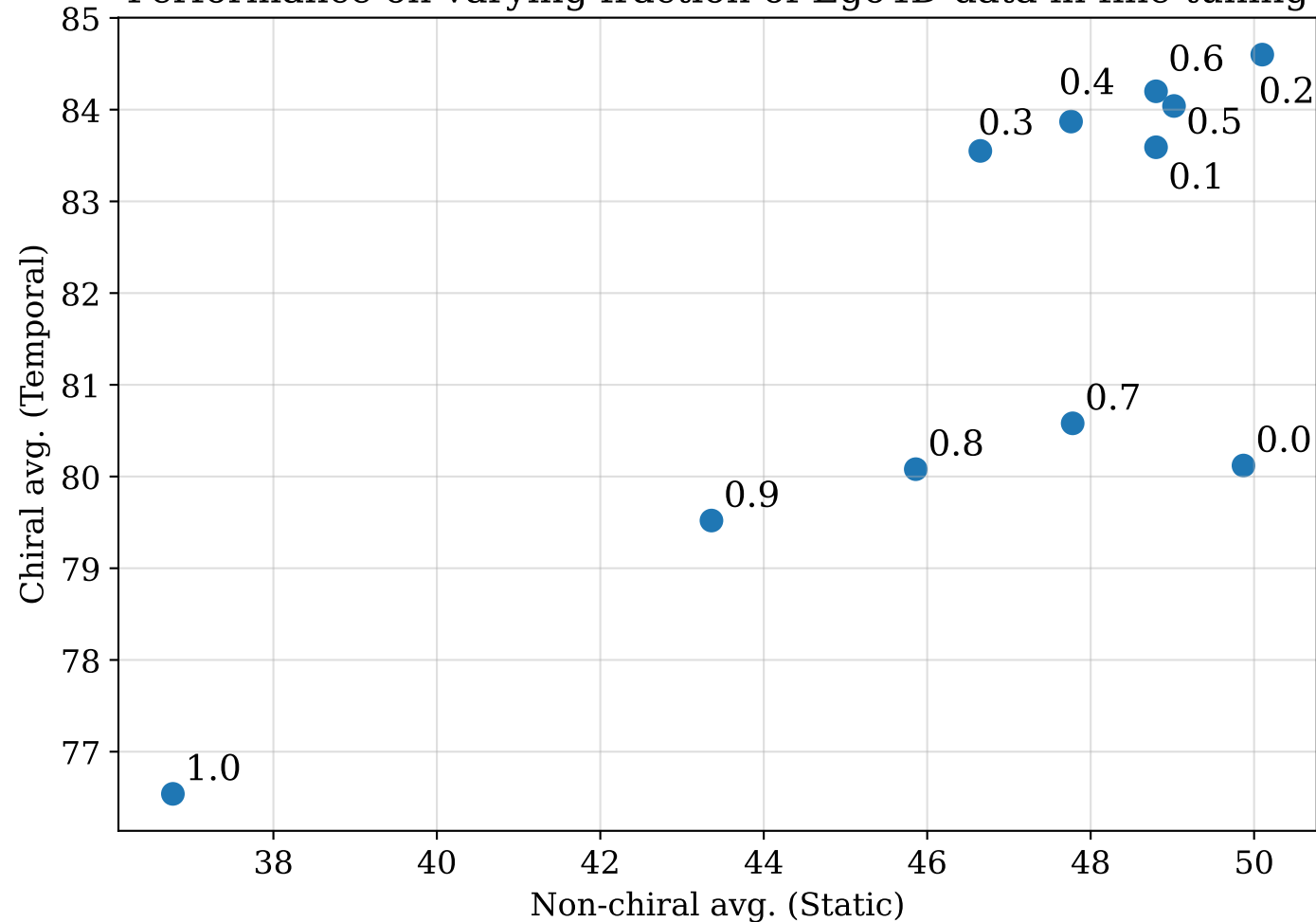
Performance on varying fraction of Ego4D data in fine-tuning
