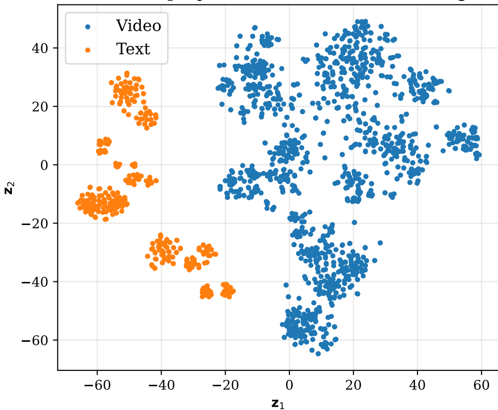
2D tSNE projection of Tarsier embeddings
