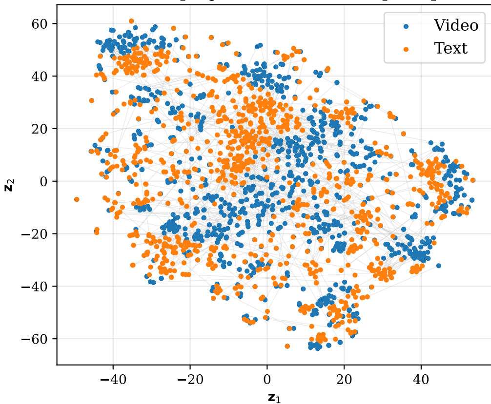
2D tSNE projection (With EOL prompt)
