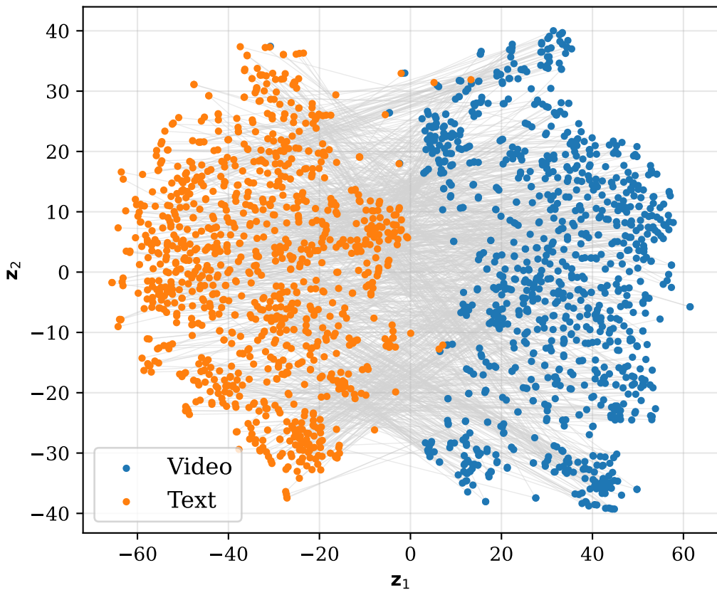
Tarsier (Base Model)
