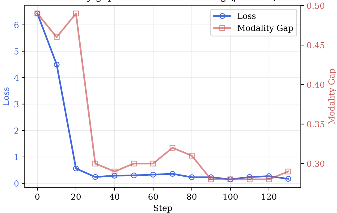
Modality gap and loss over training ( \rho = 0.77 )
