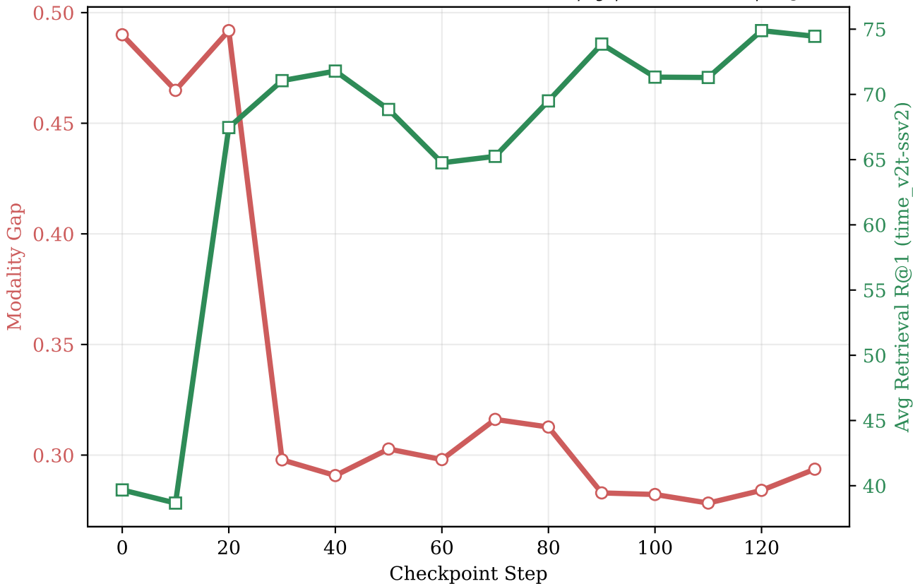
Modality Gap and Retrieval over Training ( \rho_{step, gap}=-0.75 , \rho_{step, R@1}=0.70 )
