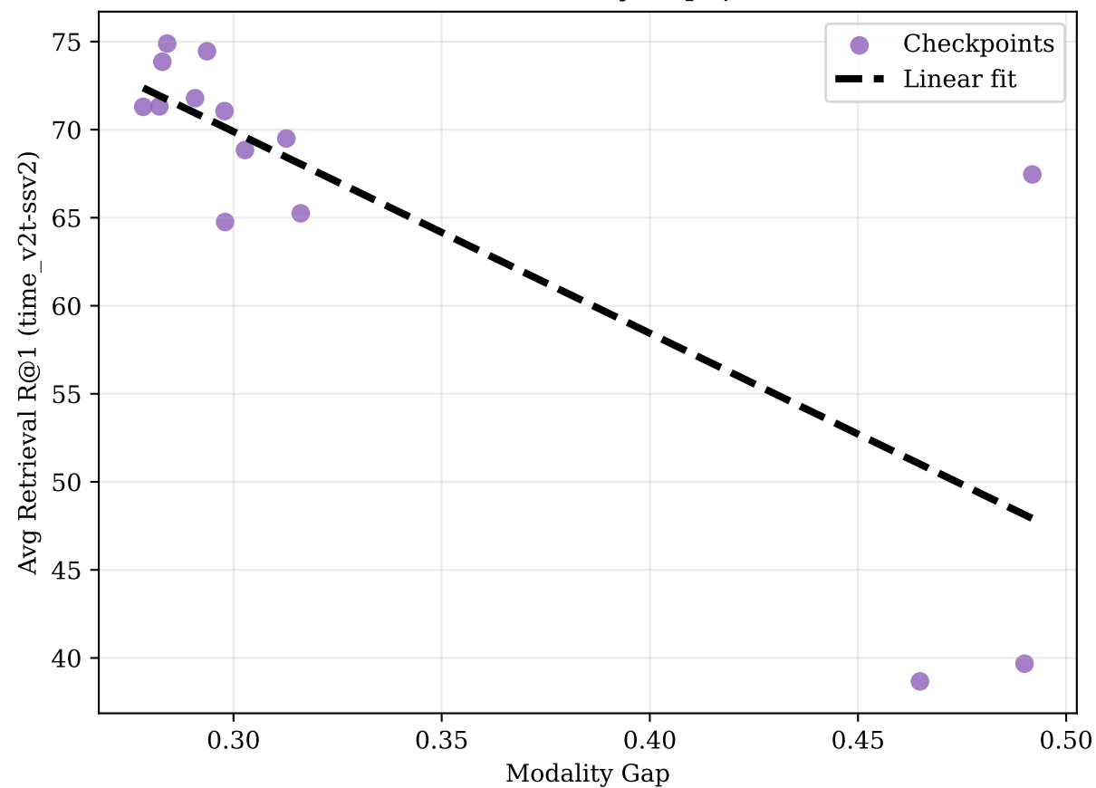
Retrieval vs Modality Gap ( \rho=-0.79 )
