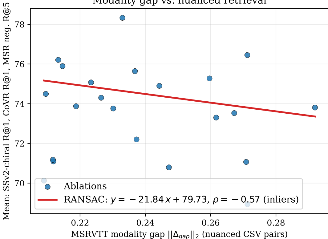
Modality gap vs. nuanced retrieval
