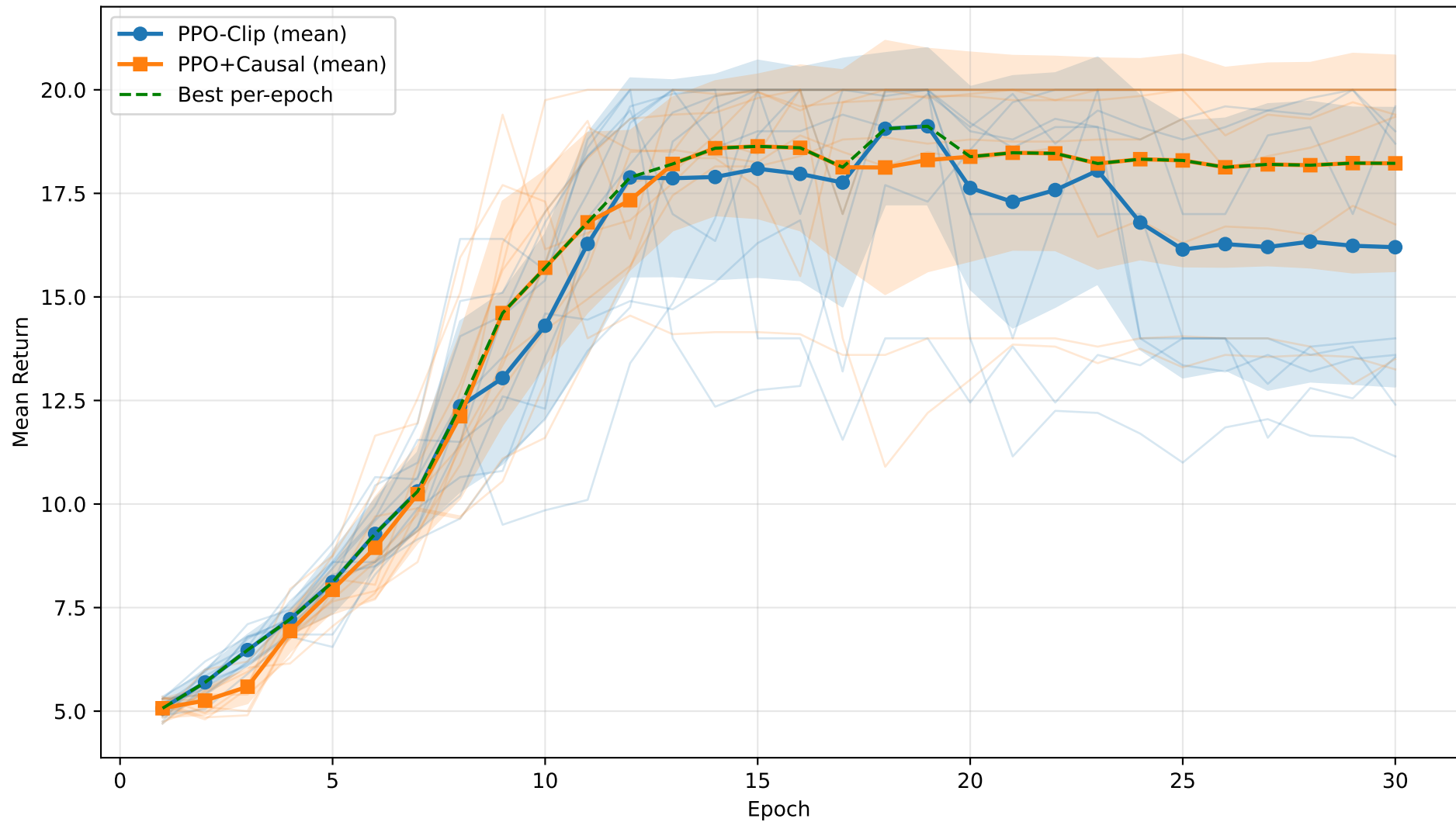
Convergence comparison — Two-Stage Assignment
