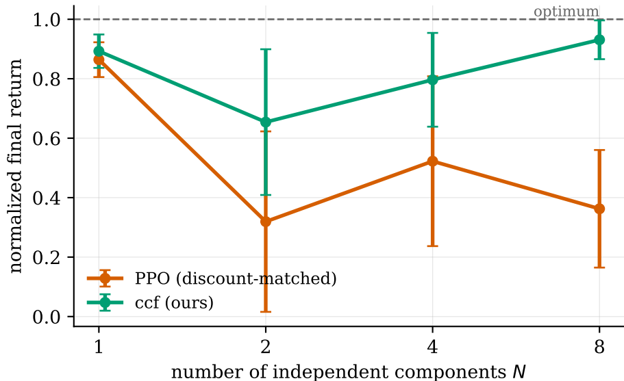
Scaling: ccf holds the optimum, PPO degrades
