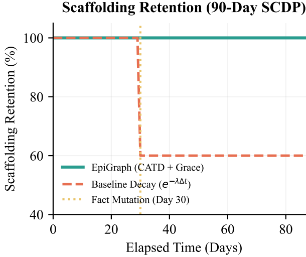
(a) Scaffolding retention over 90 simulated days.
