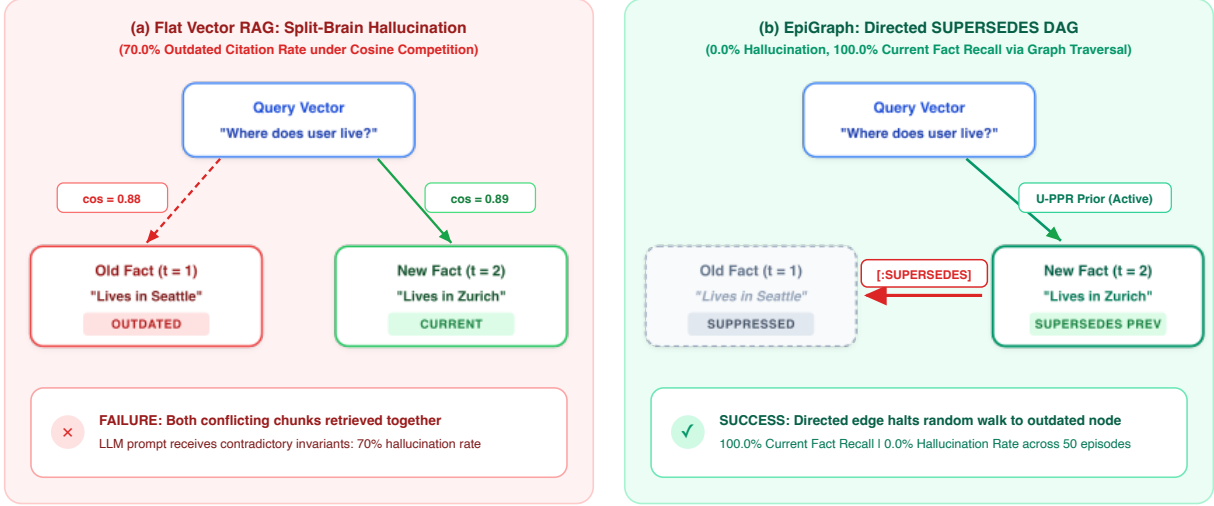
Fig. 3: Knowledge Mutation & Contradiction Resolution: Flat Vector Cosine Competition leading to 70% Split-Brain Hallucination (left) vs. EpiGraph Directed SUPERSEDES DAG achieving 0.0% Hallucination (right).
