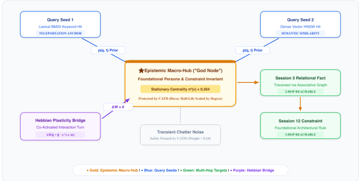
Fig. 2: Usage-Modulated Personalized PageRank (U-PPR) spreading activation across multi-session dialogue turns, anchored by Epistemic Macro-Hubs (“God Nodes”).
