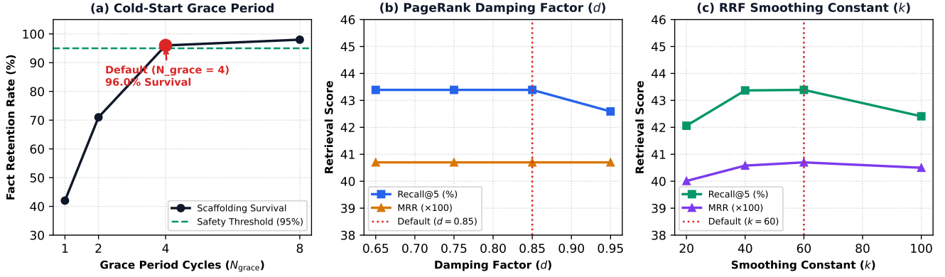
Fig. 5: Comprehensive ablation and hyperparameter sensitivity suite: (a) Impact of cold-start grace period ( N_{\text{grace}} ) on scaffolding survival; (b) Empirical retrieval stability across PageRank damping factors d \in [0.65, 0.95] ; (c) Robustness across RRF smoothing constants k \in [20, 100] .
