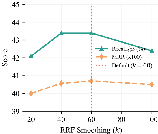
Sensitivity to RRF Constant ( k )
