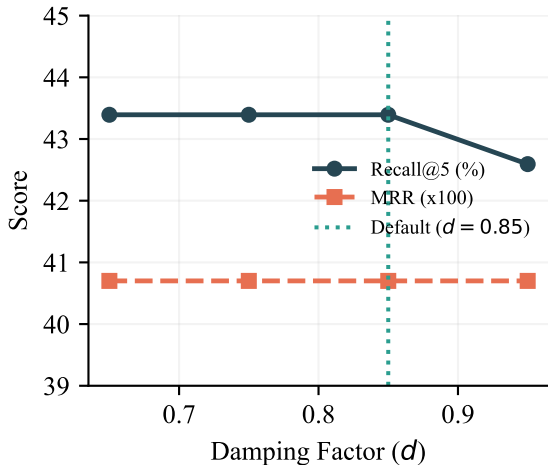
Sensitivity to PageRank Damping ( d )
