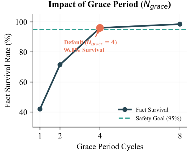
(b) Ablation of cold-start grace period ( N_{\text{grace}} ).
