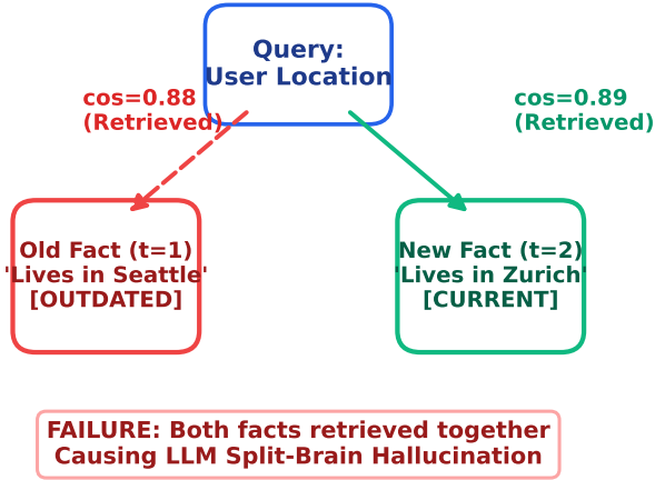
(a) Flat Vector RAG: Split-Brain Hallucination (70.0% Outdated Citation Rate)
