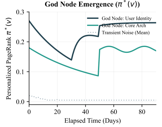
(b) God Node centrality emergence via U-PPR.
