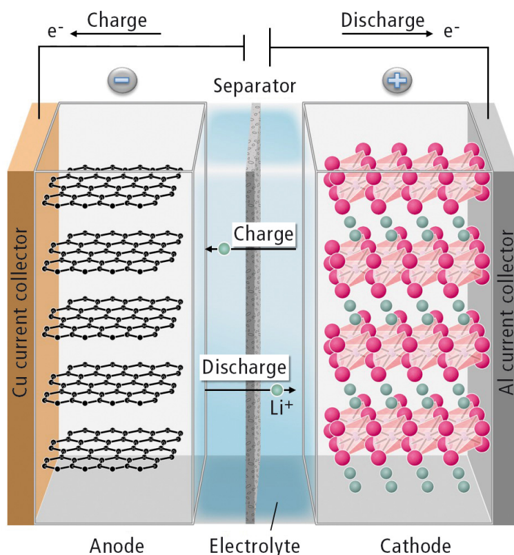
FIGURE 14.3 – Schéma simplifié d'une batterie lithium-ion. Source : C.Schultz (2016). Anti-aging for batteries ? LC-MS method development for battery electrolytes . Shimadzu News.
