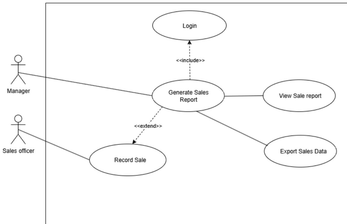
Use Case Diagram (UC-08)
