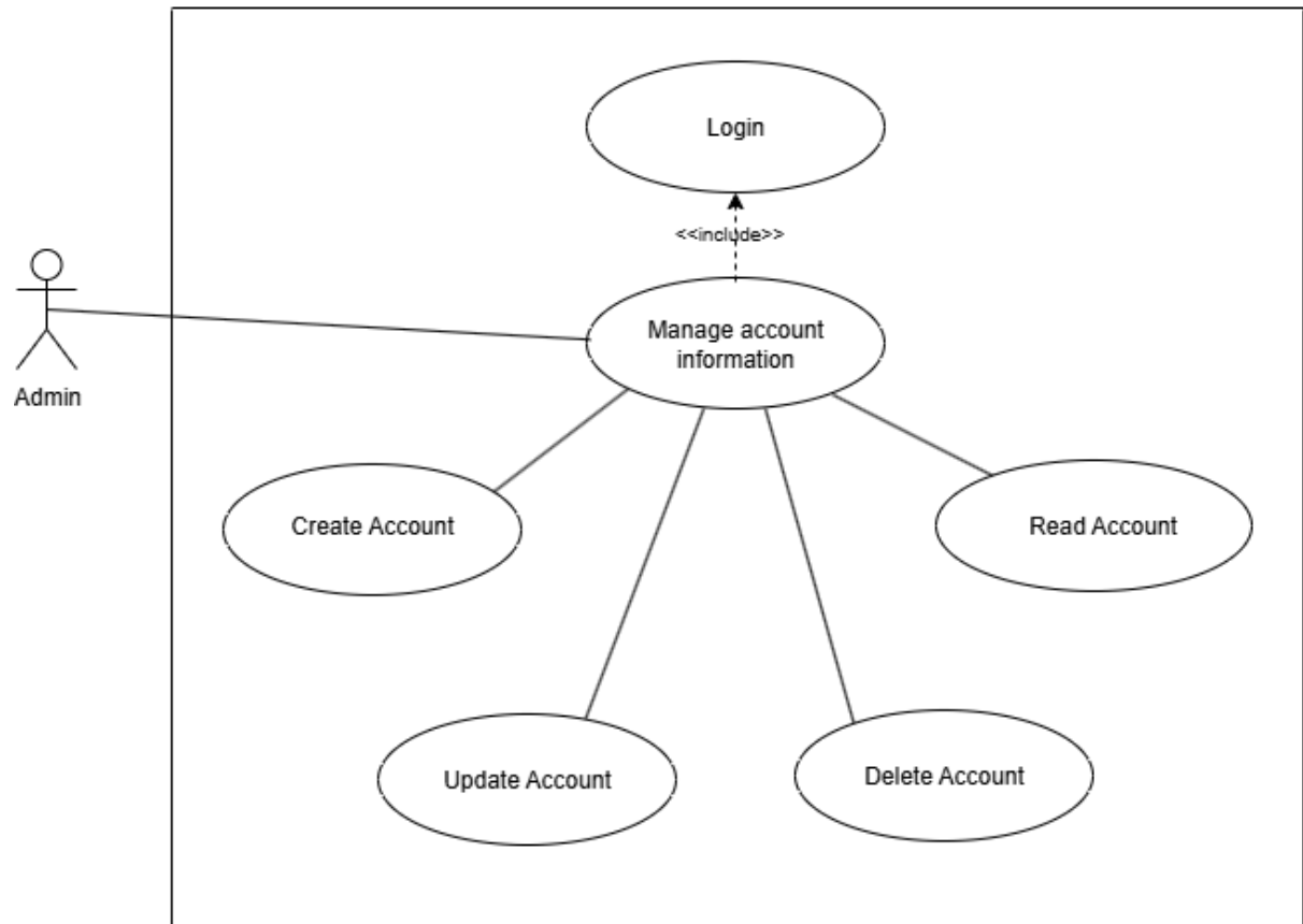
Use Case Diagram (UC-02)
