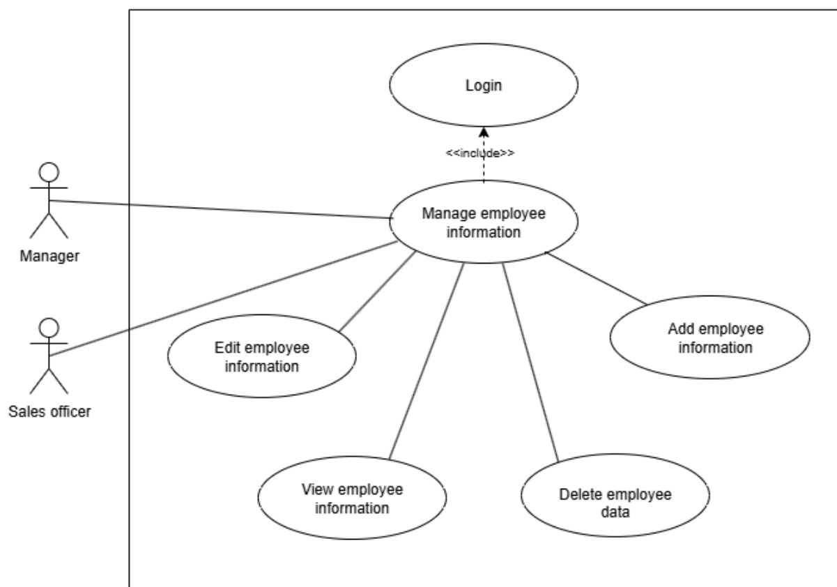
Use Case Diagram (UC-05)
