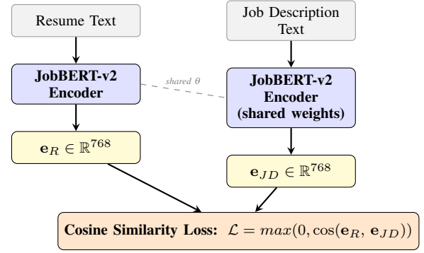
Fig. 2. Siamese encoder training architecture. Both input documents are passed through identical (weight-shared) JobBERT-v2 encoders. The cosine similarity between the resulting 768-dimensional embeddings is maximised for matched pairs and minimised for non-matched pairs during fine-tuning.
