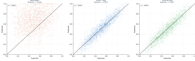
Fig. 3. Continuous similarity evaluation on 2,000 sampled instances from the 9,500-entry dataset. Predicted vs. Expected similarity scores across model variants.
