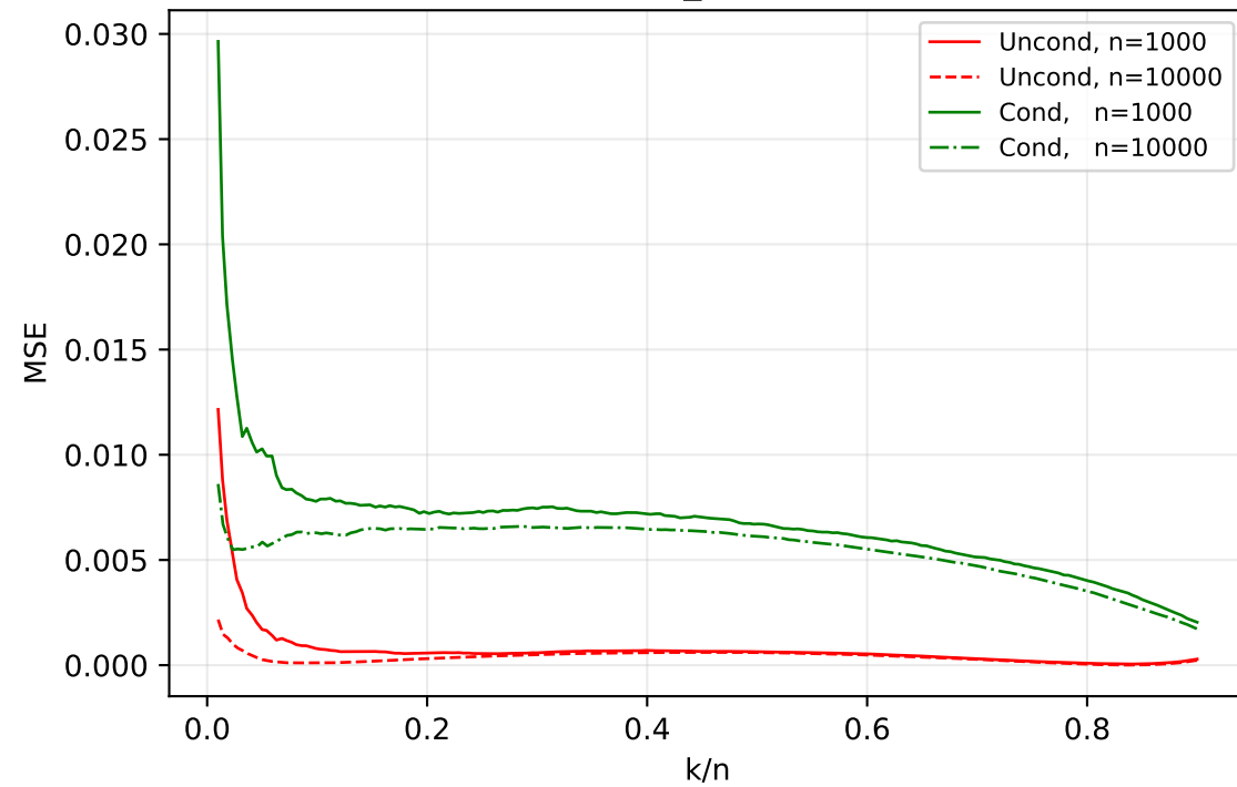
MSE, x_{\text{eval}} = 3
