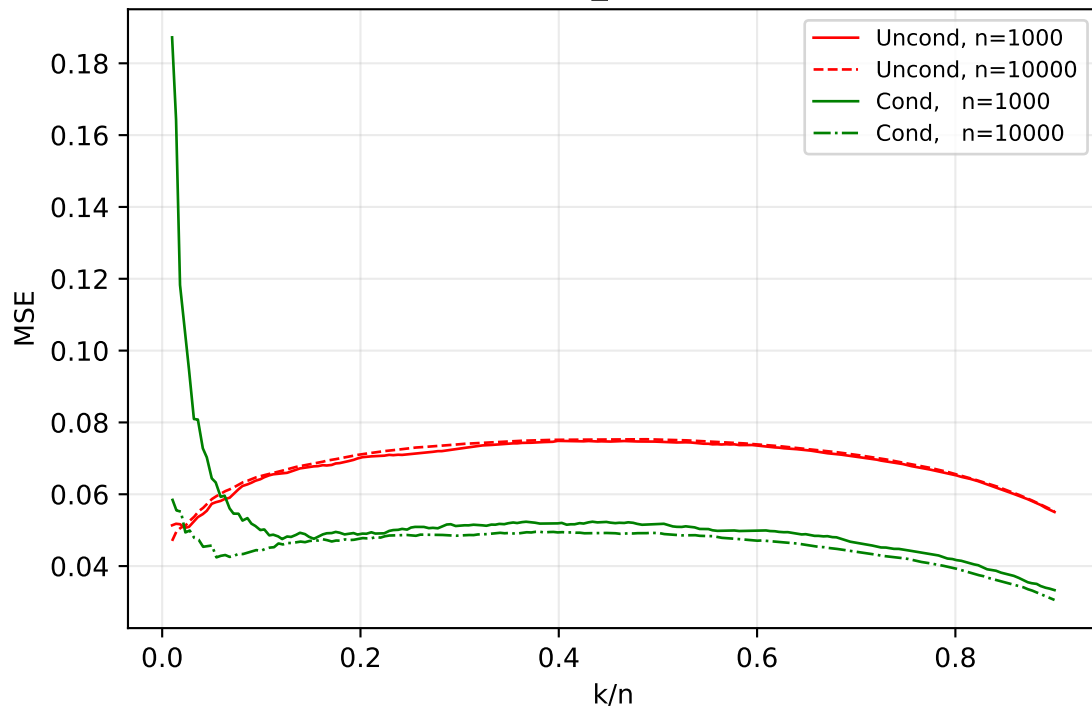
MSE, x_{\text{eval}} = 1
