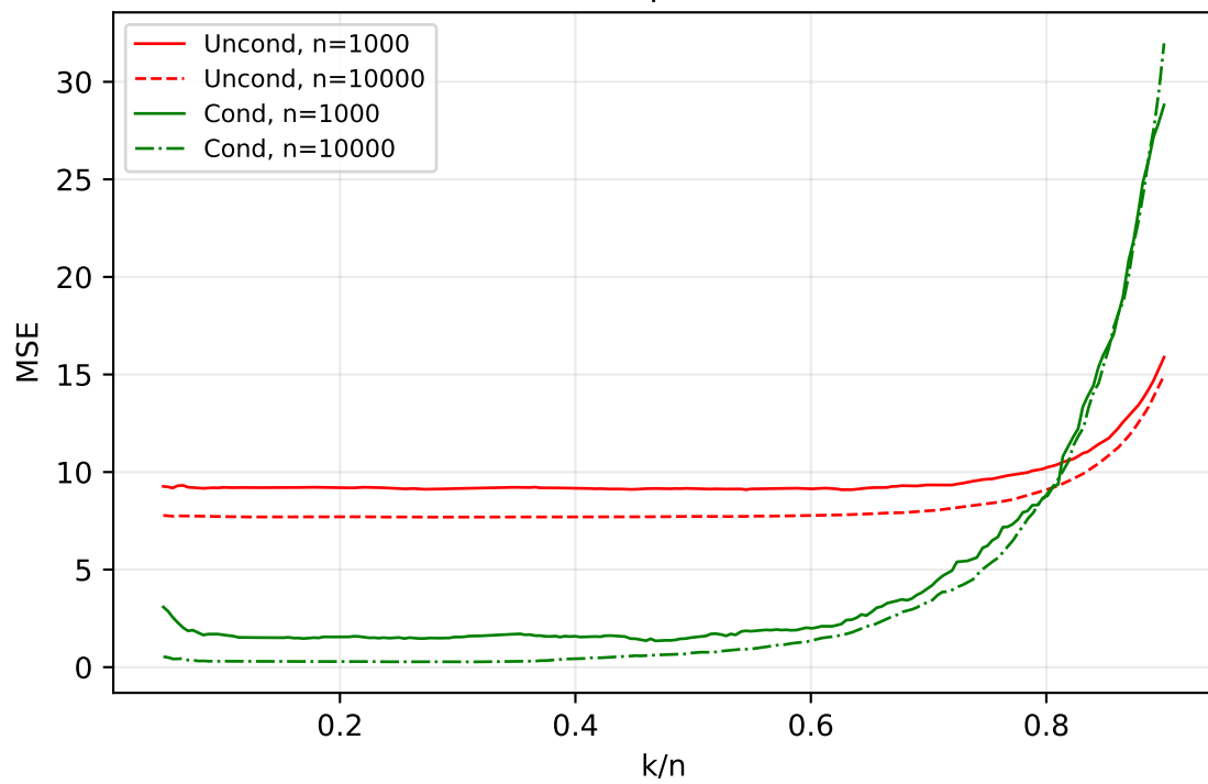
MSE, q = 0.95
