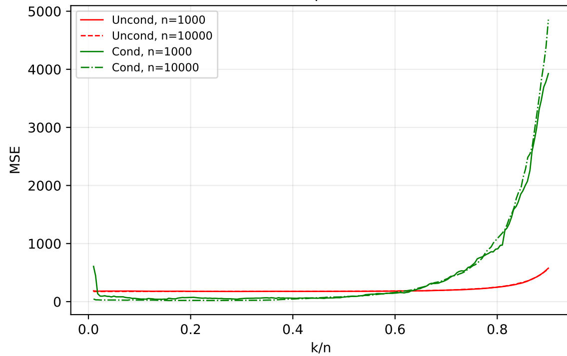
MSE, q = 0.99
