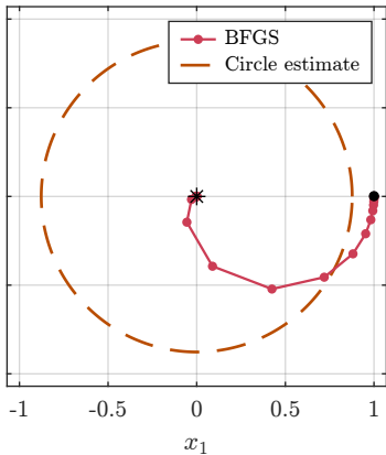
(b) BFGS: 22 iterations
