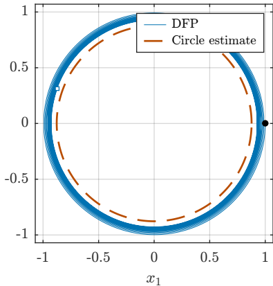
(a) DFP: 100,000 cycles
