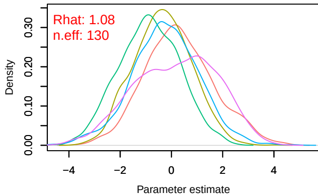
Density – mu.beta0
