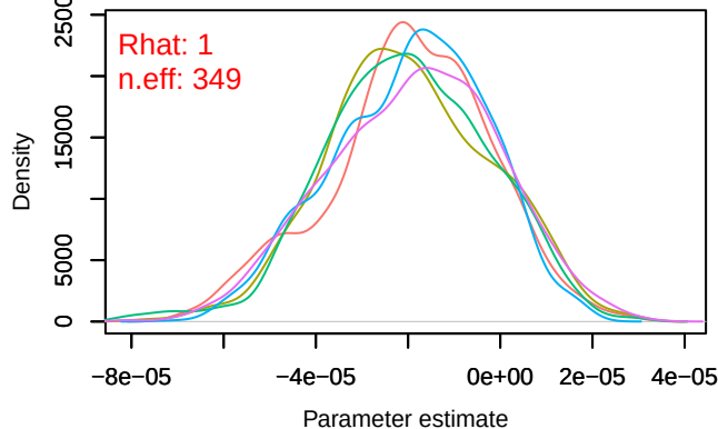
Density – alpha[1]
