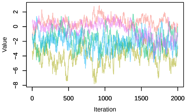
Trace – alpha[1]
