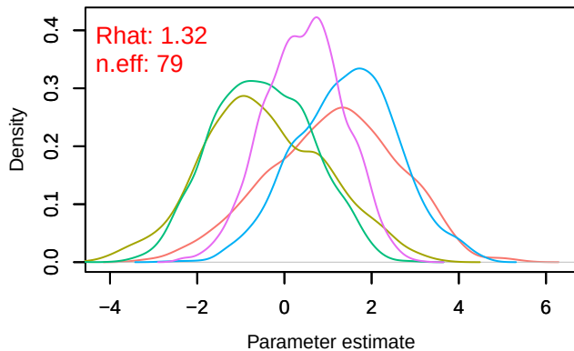
Density – mu.beta0
