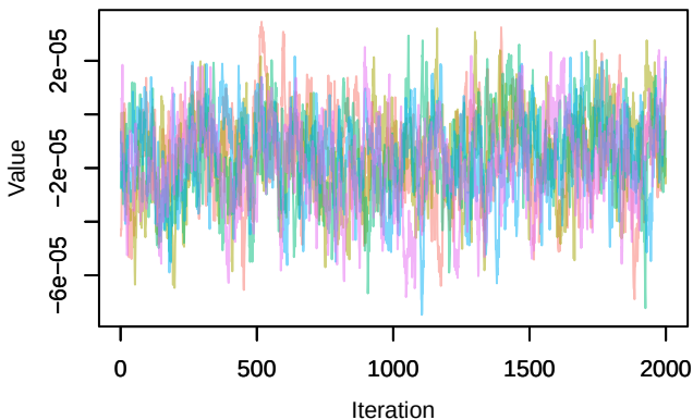
Trace – alpha[1]
