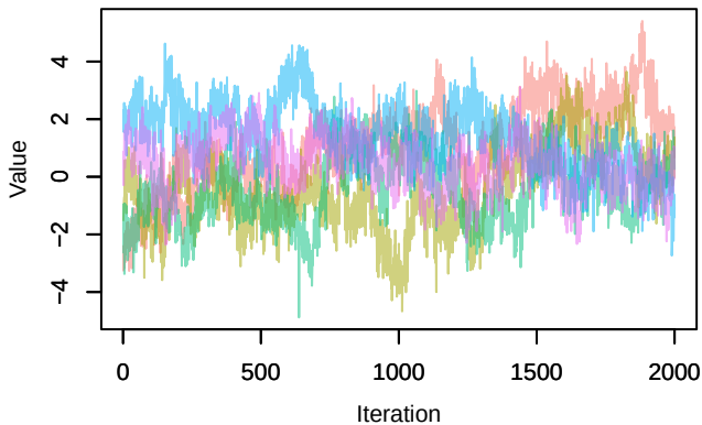
Trace – mu.beta0
