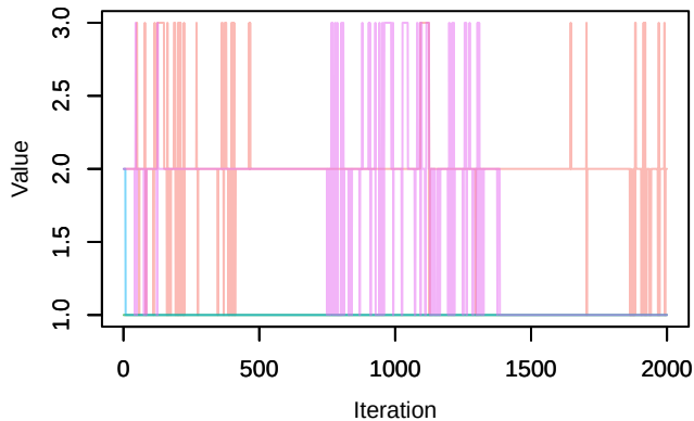
Trace – scales_beta1
