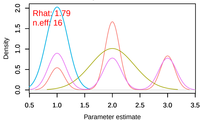
Density – scales_beta2
