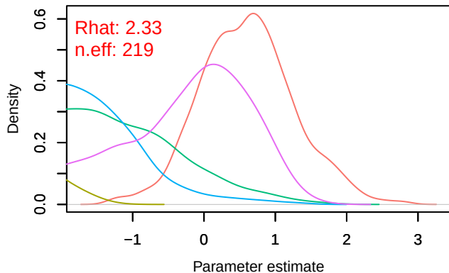
Density – alpha[1]
