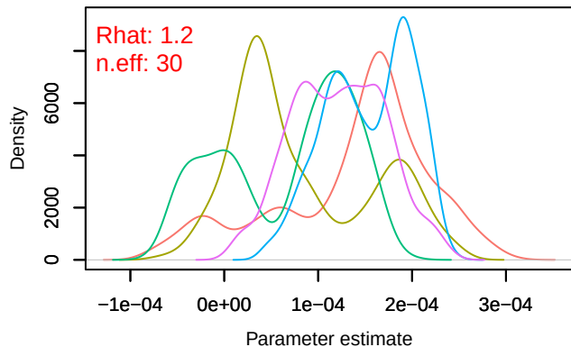
Density – scales_beta1
