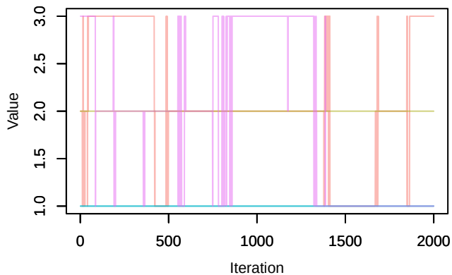
Trace – scales_beta2
