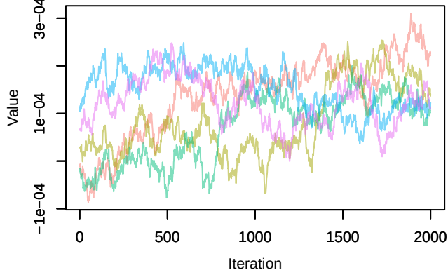
Trace – scales_beta1
