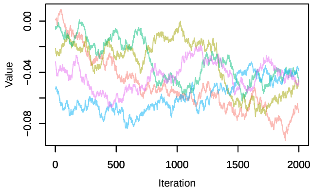
Trace – alpha[3]
