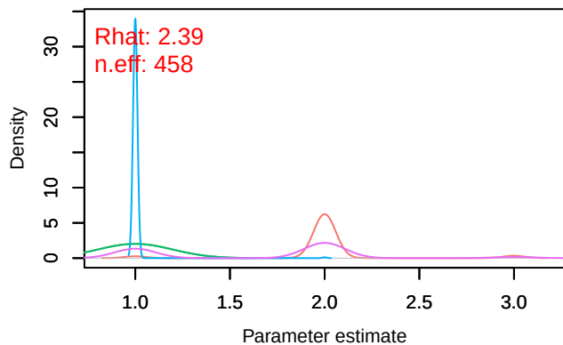
Density – scales_beta1
