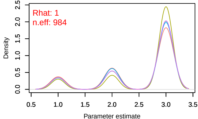
Density – scales_beta4
