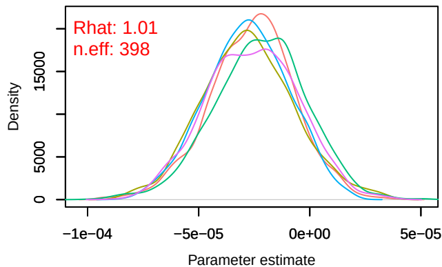
Density – alpha[1]
