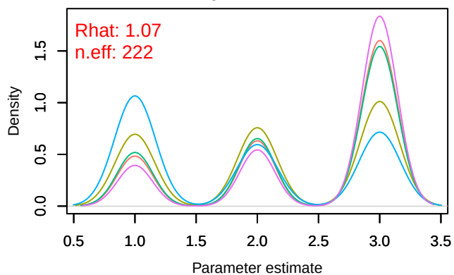
Density – scales_beta5
