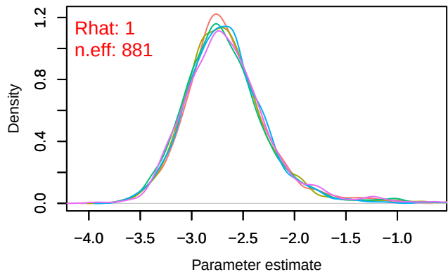
Density – beta0[3]
