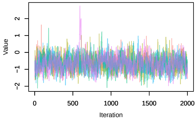
Trace – beta0[2]
