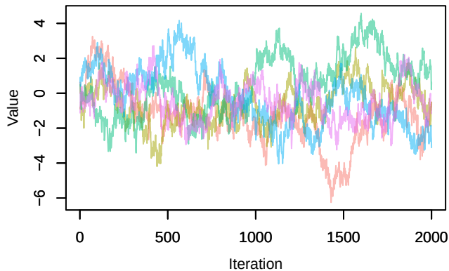
Trace – alpha0[5]
