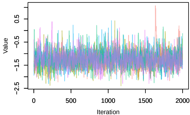
Trace – beta0[5]
