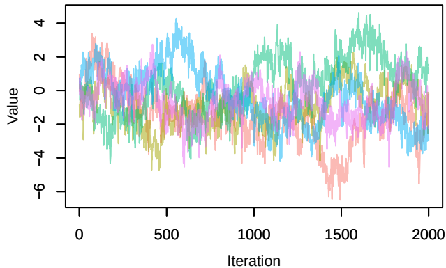
Trace – alpha0[6]
