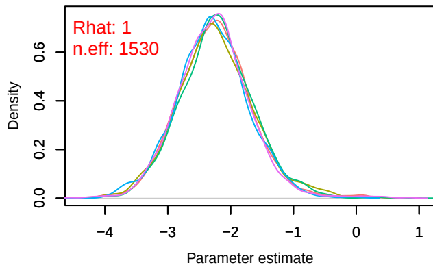
Density – beta0[6]
