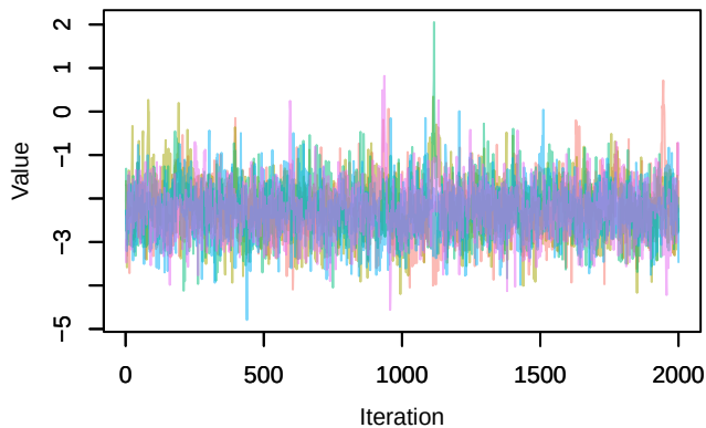
Trace – beta0[6]
