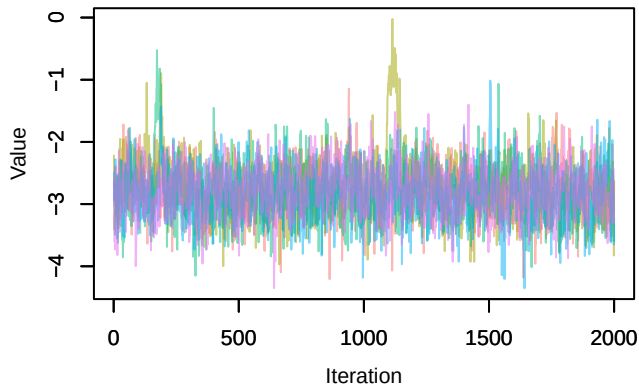
Trace – beta0[8]
