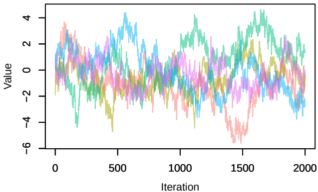
Trace – alpha0[8]
