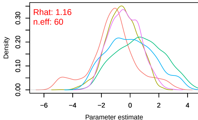
Density – alpha0[3]
