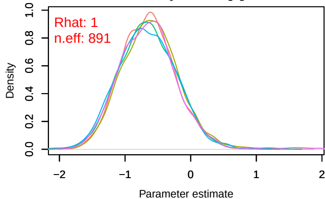
Density – beta0[2]
