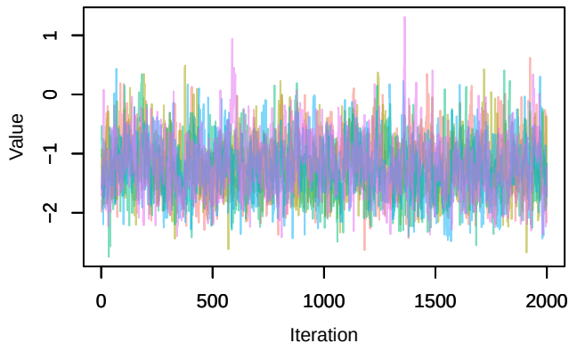
Trace – beta0[3]
