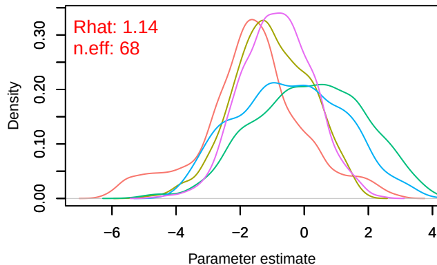
Density – alpha0[6]
