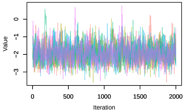
Trace – beta0[6]
