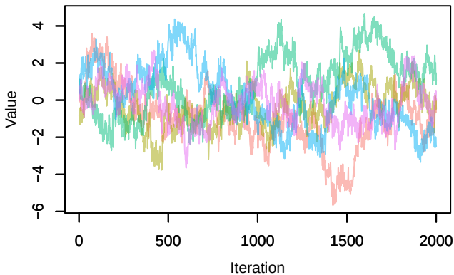
Trace – alpha0[2]
