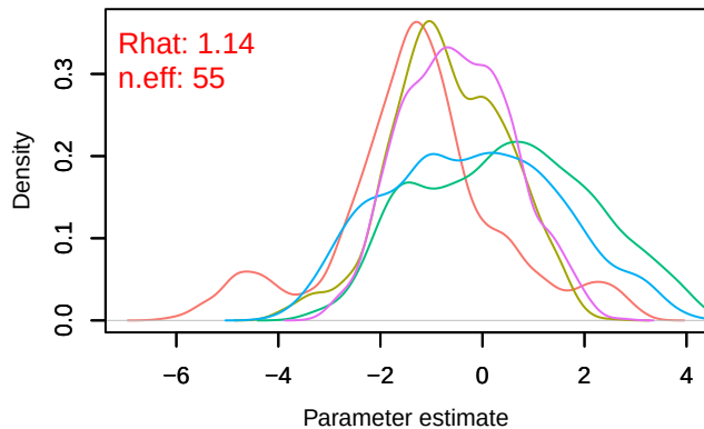
Density – alpha0[5]
