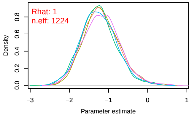
Density – beta0[3]
