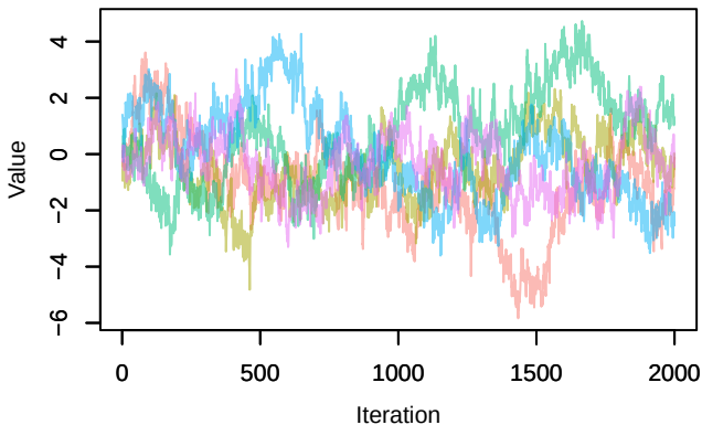
Trace – alpha0[3]
