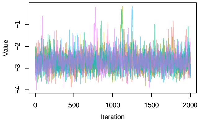
Trace – beta0[3]
