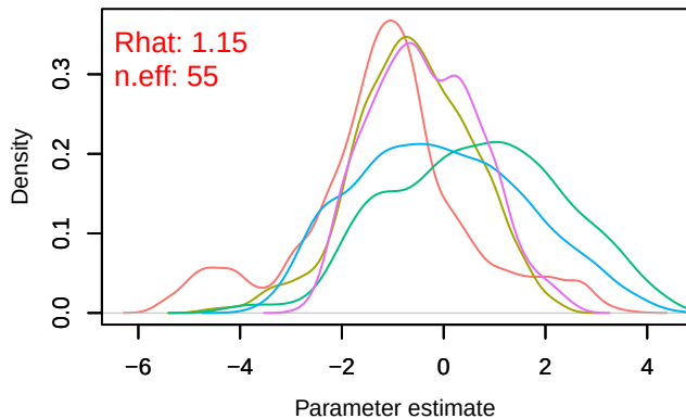
Density – alpha0[8]
