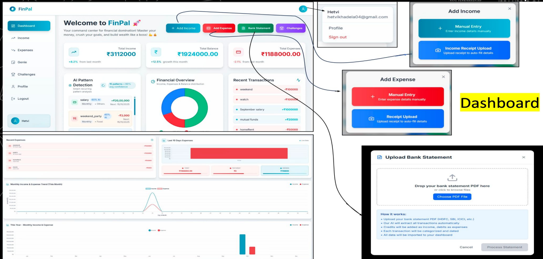
Screenshot 2 (Dashboard)
