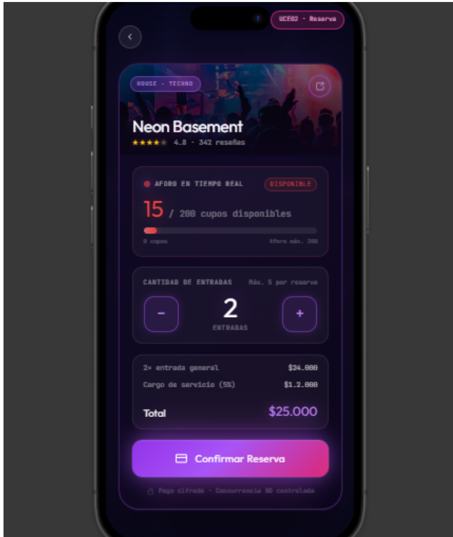
Figura 4: Mockup Conceptual - CU02: Reserva y Pago (Transaccional)
