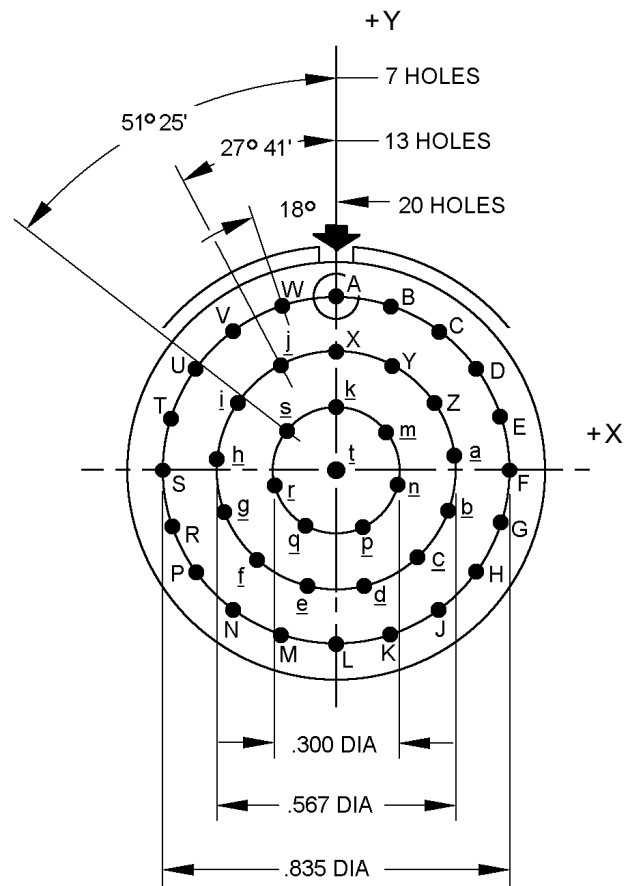
FIGURE 7. Insert arrangement, electrical connector, shell size 21 (series I, III, IV of MIL-DTL-38999, series I of MIL-DTL-27599, and series A of SAE-AS29600) – Continued.
