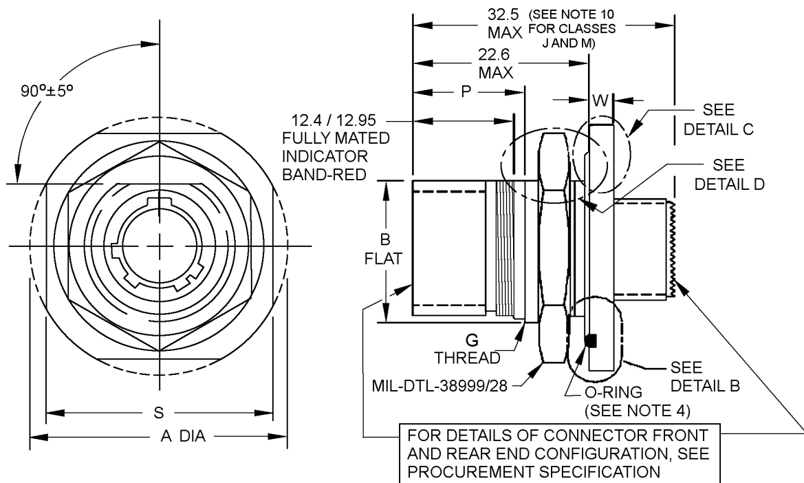
FIGURE 1. Receptacle.
