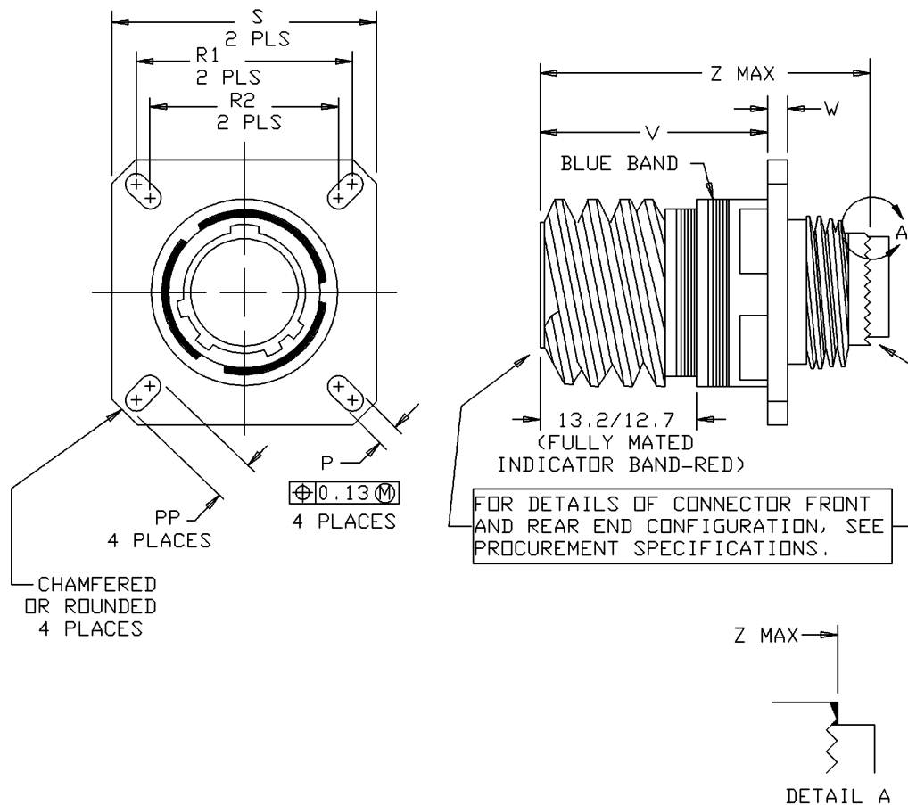
FIGURE 1. Receptacle, fiber optic.
