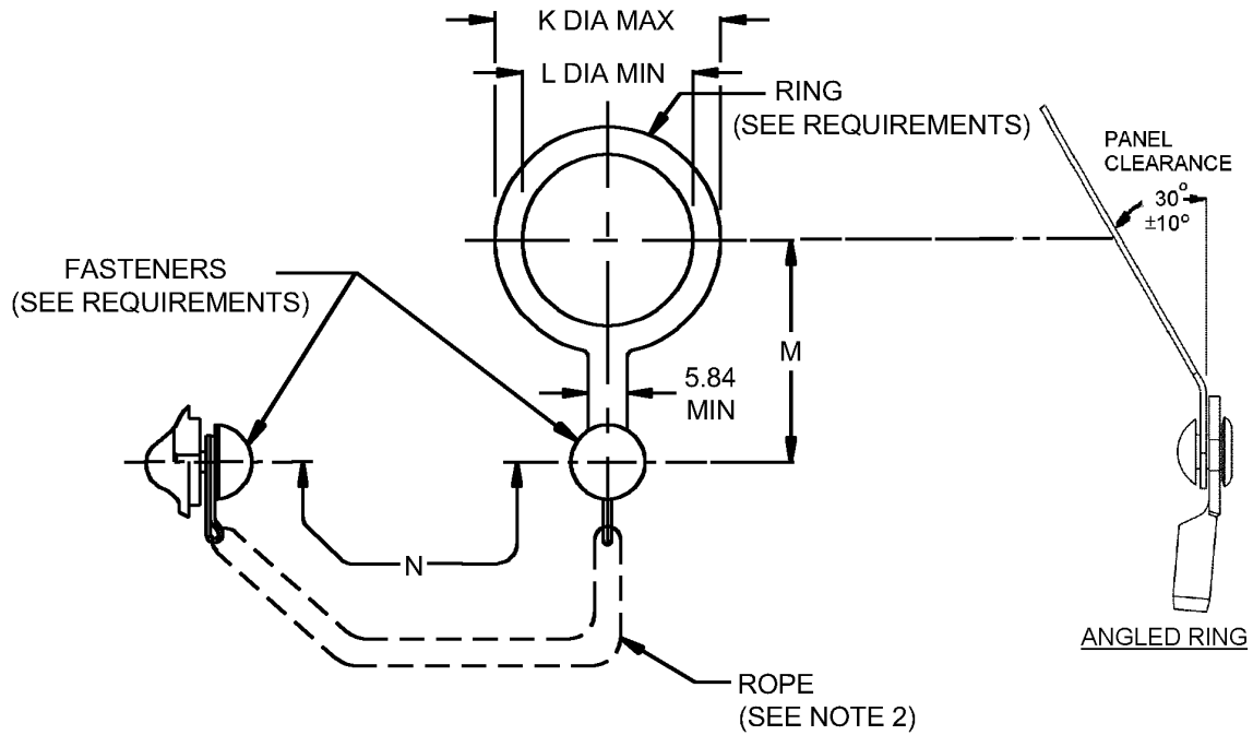
STYLE N (WITH ROPE AND RING)
