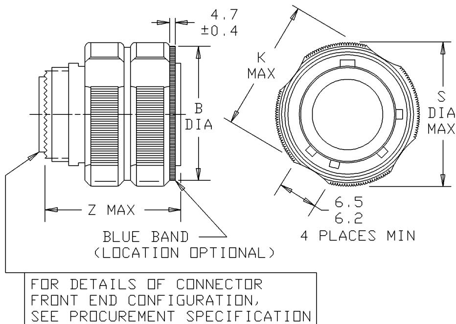
FIGURE 1. Plug, fiber optic.
