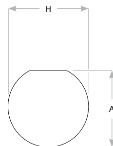
Panel Cutout
