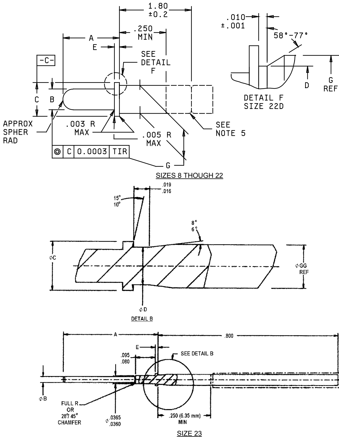
FIGURE 16. Test gauge, pin, gauge location, and retention (all series).
